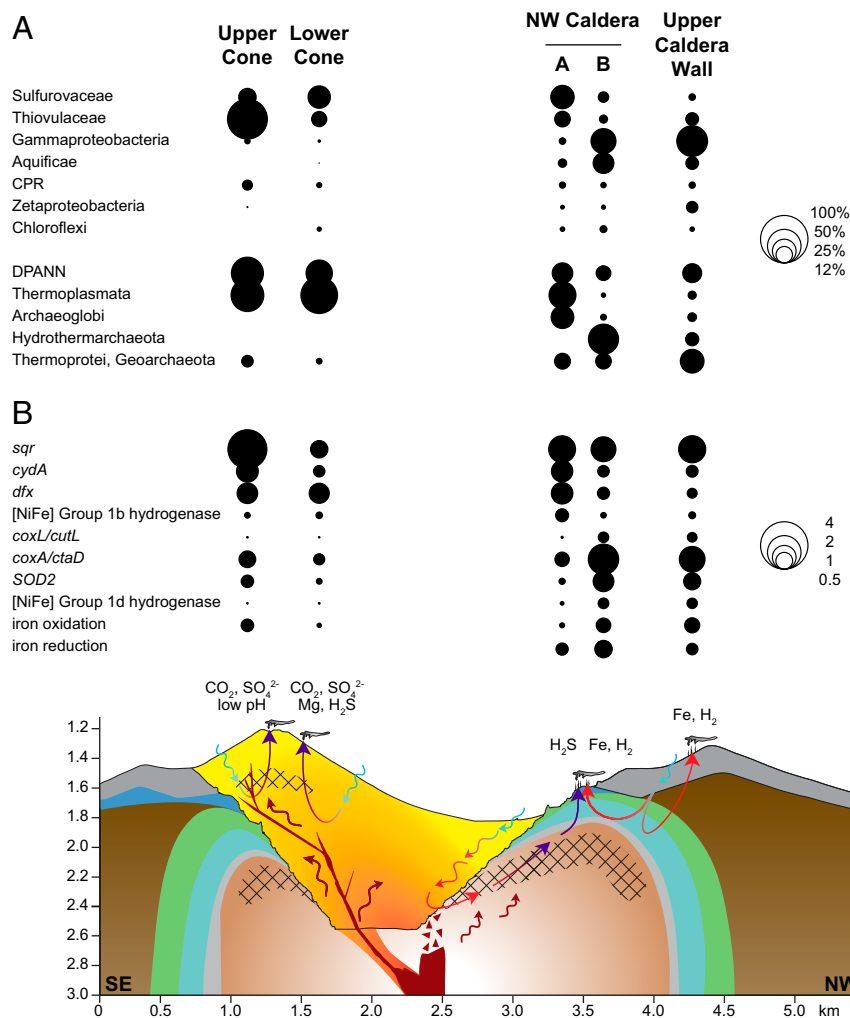
Fig. 6. The proposed influence of subsurface hydrogeological processes on the microbial phylogenetic and functional diversity associated with Brothers volcano and its hydrothermal systems. Schematic cross-section adapted from de Ronde et al. (9) from southeast to northwest. Overall, the shallow subsurface is influenced by seawater-dominated hydrothermal circulation (blue arrows = recharge; red arrows = discharge). Recharge of seawater occurs both at a volcano scale through the caldera floor and faults along the caldera wall and more locally at the 100- to 200-m scale at the vent sites [see Caratori Tontini et al. (35)]. Red arrows denote heated (modified) seawater after reaction with the rocks; purple arrows represent hot, magmatically influenced fluids; red-brown arrows represent magmatic volatiles. Cross-hatching represents zones of inferred magmatic salt [see de Ronde et al. (9)]. (A) Bubble plots of the average relative abundance of key taxa (NCBI taxonomy) amplicons discussed in the text from each area are shown, with bubble size corresponding to percent average relative abundance (Dataset S1C; UC, n = 3 samples; LC, n = 2 samples; NWC-A, n = 6 samples; NWC-B, n = 3 samples; UCW, n = 2 samples). The average relative abundance of Archaea was calculated separately using only archaeal taxa, and bubble size represents the percent average relative abundance of Archaea (UC, n = 2 samples; LC, n = 2 samples; NWC-A, n = 6 samples; NWC-B, n = 3 samples; UCW, n = 2 samples). (B) Associated enrichment of key functional genes where bubble size corresponds to relative abundances as described for Fig. 3A (Dataset S2B), averaged across samples at each area. Enrichment of carbon dioxide ( \text{CO}_2 ), sulfate ( \text{SO}_4^{2-} ), magnesium (Mg), hydrogen sulfide ( \text{H}_2\text{S} ), iron (Fe) and hydrogen ( \text{H}_2 ) and pH shifts are shown for each site (Dataset S1B). The combination of different geochemical environments intersected by the circulating hydrothermal fluids, and different scales of recharge, may explain some of the shifts in diversity of the microbial communities observed at Brothers volcano.
