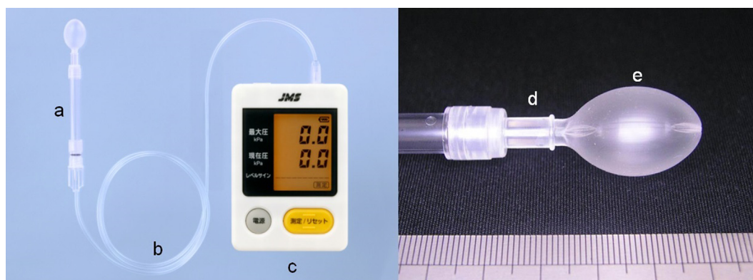
Figure 1 JMS tongue pressure measurement device. This device consists of a) disposable oral probe, b) tube, and c) digital device (TPM-01). The probe consists of d) hard plastic ring and e) air-filled balloon.
