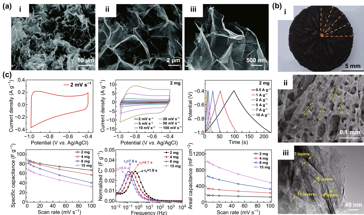
Fig. 6 Ti_3C_2T_x aerogel. a SEM image of the Ti_3C_2T_x aerogel with different magnifications [40]. b Cross-sectional view of Ti_3C_2 aerogel, SEM image of Ti_3C_2 aerogel, and TEM of void walls. c CV and GCD curves of Ti_3C_2 aerogel, specific capacitance with different mass loadings, progression of the imaginary ( C'' ) parts of the stack capacitance of Ti_3C_2 aerogel and areal capacitance with different mass loadings [96]. Reproduced with permission from Refs. [40, 96]
