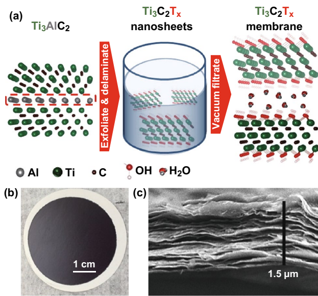
Fig. 2 a A schematic of the synthesis of a Ti_3C_2T_x membrane, b photograph, and c SEM image of cross-sectional of the Ti_3C_2T_x membrane. Reprinted with the permission from Ref. [36]. Copyright © (2015) American Chemical Society
