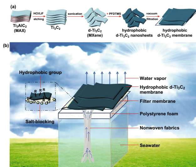
Fig. 13 Schematic illustration of a fabrication process of the hydrophobic d\text{-Ti}_3\text{C}_2 membrane, and b the hydrophobic d\text{-Ti}_3\text{C}_2 membrane-based solar desalination device. Reprinted with permission from Ref. [72]. Copyright © (2019) Royal Society of Chemistry
