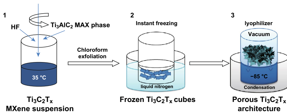
Fig. 12 Synthetic procedure for the porous \text{Ti}_3\text{C}_2\text{T}_x architecture. Reprinted with permission from Ref. [62] Copyright © (2018) Elsevier Inc
