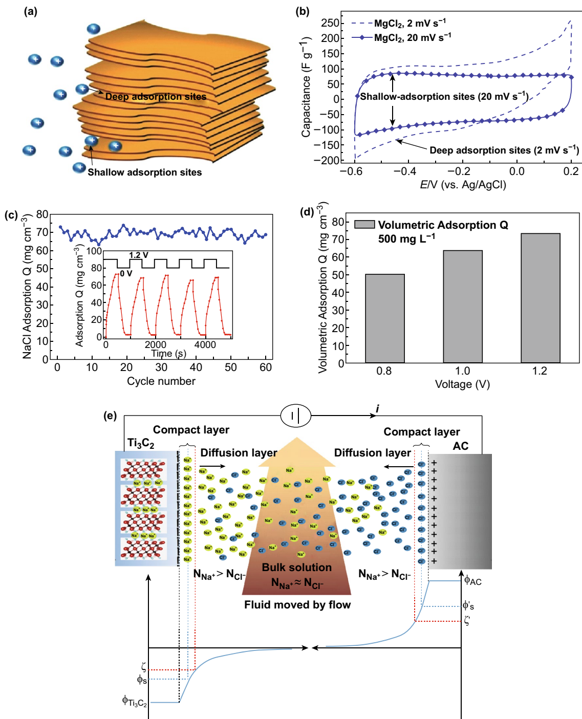
Fig. 11 a Schematic illustration of multilayered \text{Ti}_3\text{C}_2\text{T}_x particle containing shallow and deep adsorption sites near the gap opening and in its interior, respectively, b Capacitance of \text{Ti}_3\text{C}_2\text{T}_x/\text{carbon black-PTFE} laminate in a Swagelok cell measured at scan rates of 2 and 20 \text{ mV s}^{-1} (dashed line and symbols, respectively) in 1 \text{ M MgCl}_2 related to deep and shallow adsorption sites, respectively. Reprinted with permission from Ref. [66]. Copyright © (2015) John Wiley & Sons, Inc. c Electroadsorption and regeneration cycles of porous \text{Ti}_3\text{C}_2\text{T}_x electrode in 500 \text{ mg L}^{-1} NaCl solution. d Electroadsorption capacitance of porous \text{Ti}_3\text{C}_2\text{T}_x at varied voltage in 500 \text{ mg L}^{-1} NaCl solution. Reprinted with permission from Ref. [62]. Copyright © (2018) Elsevier Inc. e Schematics of the CDI process. Reprinted with permission from Ref. [60]. Copyright © (2018) Elsevier B.V
