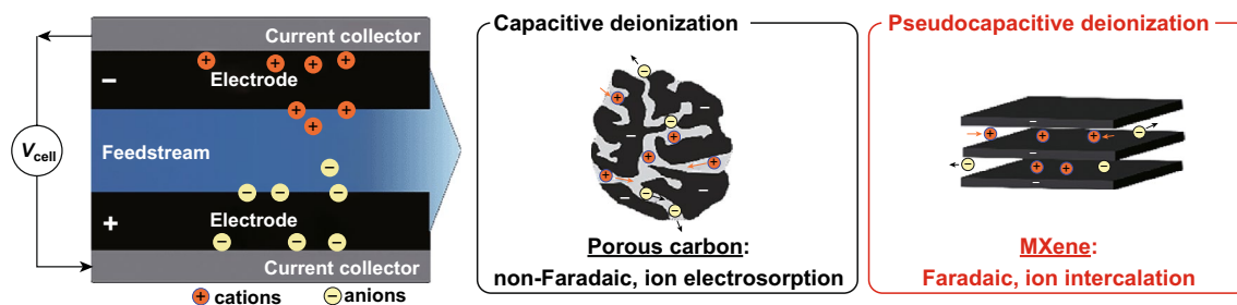
Fig. 10 Concept of electrochemical water desalination by non-faradaic (electrostatic) ion electrosorption at the surface of electrode materials. Reprinted with permission from Ref. [39]. Copyright © (2019) Royal Society of Chemistry
