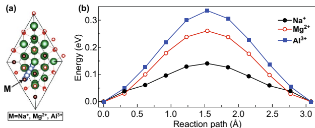
Fig. 5 a Considered ion migration pathway and b corresponding energy profiles of Na^+ , Mg^{2+} , and Al^{3+} . Reprinted with permission from Ref. [52]. Copyright © (2019) AIP Publishing LLC
