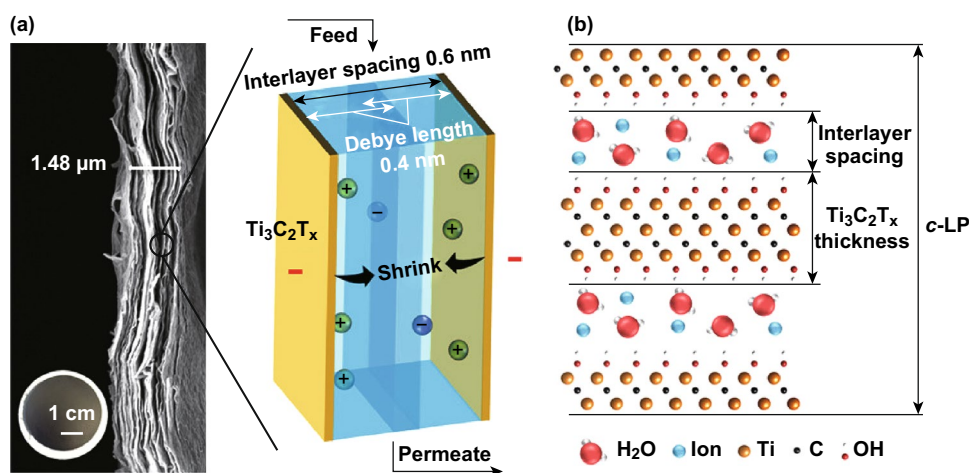
Fig. 9 a Cross-sectional SEM image of a \text{Ti}_3\text{C}_2\text{T}_x membrane with a schematic showing the interaction between \text{Ti}_3\text{C}_2\text{T}_x layers and ions within their EDLs when the \text{Ti}_3\text{C}_2\text{T}_x membrane is connected to a negative voltage. b Molecular model of \text{Ti}_3\text{C}_2\text{T}_x showing two layers of water with ions between the layers. The c lattice parameter ( c -LP) calculated from XRD is two \text{Ti}_3\text{C}_2\text{T}_x flake thicknesses and two interlayer spacings. Reprinted with permission from Ref. [59]. Copyright © (2018) American Chemical Society
