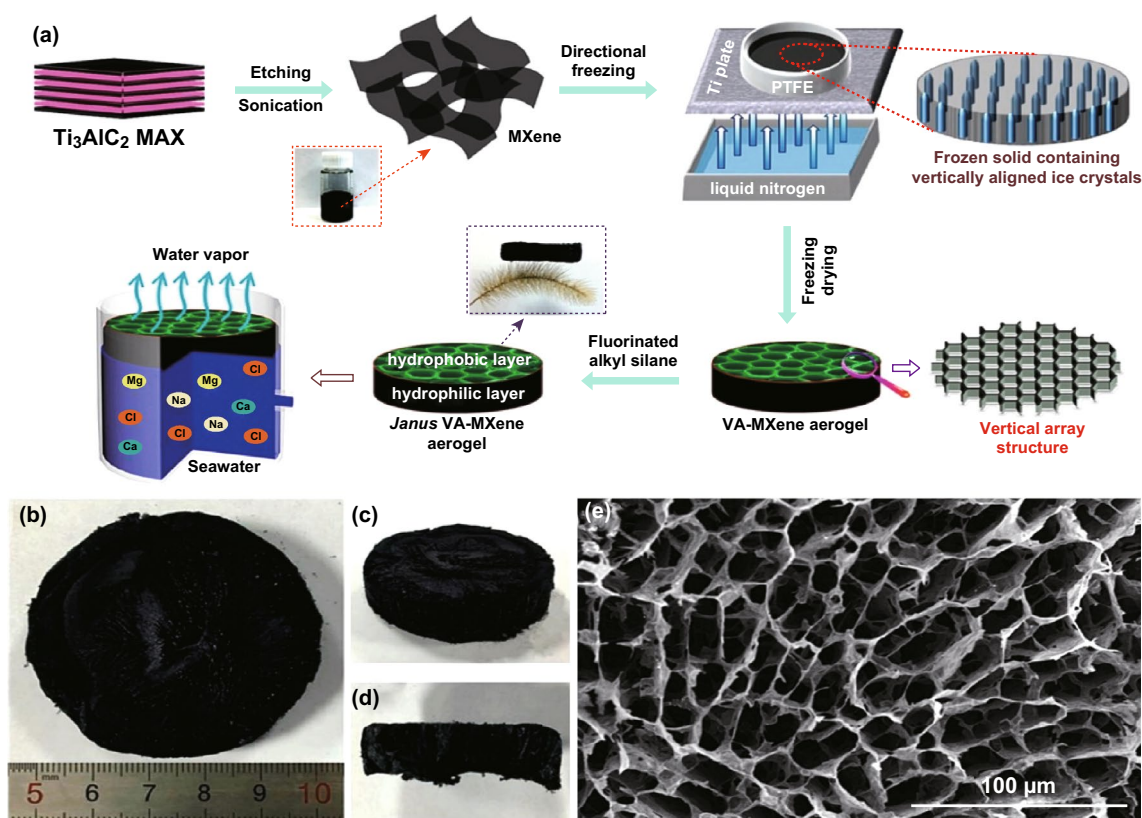
Fig. 15 a Fabrication process of a Janus VA-MXA with vertically aligned channels. b Digital photograph of the top view of the as-prepared Janus VA-MXA. c Photograph of the side view. d Photograph of the fracture face. e SEM images of the upper layer of prepared Janus VA-MXA. Reprinted with permission from Ref. [74]. Copyright © (2019) American Chemical Society
