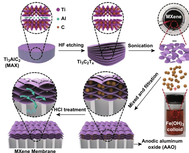
Fig. 6 Schematic of MXene membrane preparation via HF etching and intercalation by using Fe(OH)_3 colloidal solution. Reprinted with permission from Ref. [53]. Copyright © 2017 John Wiley & Sons, Inc
