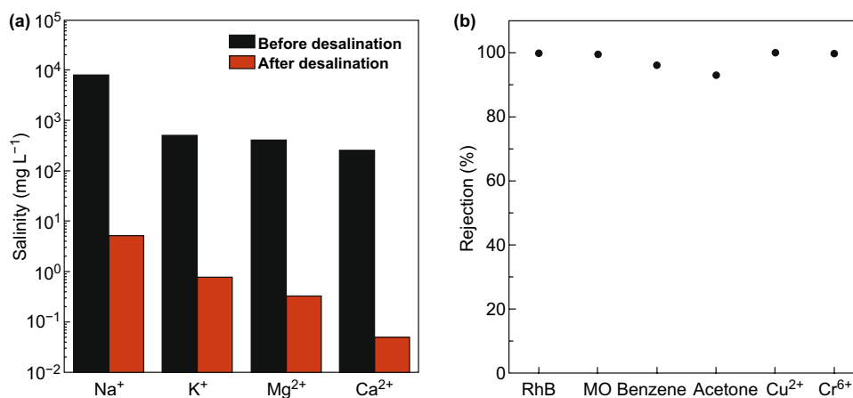
Fig. 14 a Measured salinity of four primary ions before and after solar desalination. b Organic and heavy metal ion rejection performance. Reprinted with permission from Ref. [72]. Copyright © (2019) Royal Society of Chemistry
