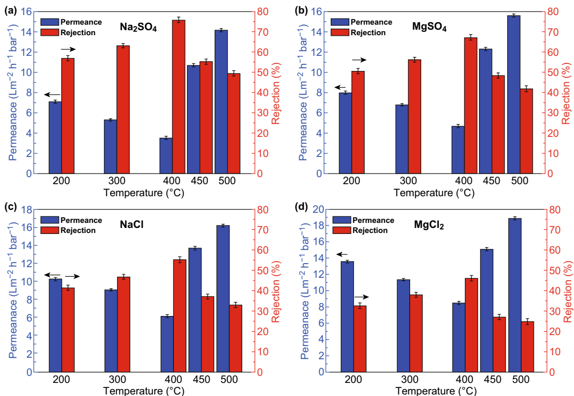
Fig. 7 a–d Rejections and salt permeances of the MXene membranes. Reprinted with permission from Ref. [54]. Copyright © (2019) Elsevier B.V
