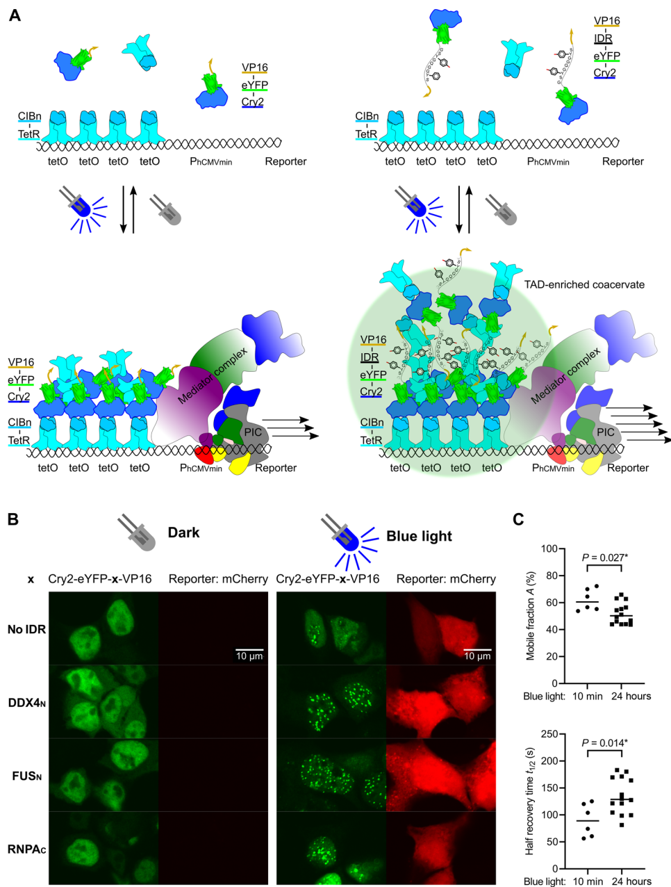
Fig. 2. Design of droplet optogenetic transcription factors (OptoTF). (A) Left: Conventional optogenetic TFs. CIBn-TetR is continuously bound to tetO. Upon blue light illumination, Cry2-eYFP-VP16 (OptoTF-) is recruited to the promoter via heterodimerization of Cry2 and CIBn. Homomultimerization of Cry2 leads to further accumulation of the TAD VP16, resulting in high expression of the reporter gene. Right: Droplet optogenetic TFs (Cry2-eYFP-IDR-VP16, OptoTF + IDR). Blue light triggers coacervate formation of OptoTF + IDR due to binding to CIBn-TetR and homo-oligomerization of Cry2. The resulting locally increased TAD concentration further increases reporter gene expression. (B) Light-responsive distribution of OptoTF- and different OptoTF + IDRs in HEK-293 cells. OptoTF- or OptoTF + IDR with three different IDRs (DDX4, FUS, and hnRNP1) was cotransfected with a tetO 13 -based mCherry reporter and analyzed by fluorescence microscopy after 24-hour cultivation in the dark (left) or under blue light (465 nm, 5 μmol m -2 s -1 ). (C) Mobile fractions and half-recovery times of OptoTF + FUS droplets determined by fluorescence recovery after photobleaching (FRAP). OptoTF + FUS, CIBn-TetR, and a tetO 7 -based reporter were cotransfected into HEK-293 cells. Cells were illuminated with blue light (465 nm, 5 μmol m -2 s -1 ) for either 10 min or 24 hours before measurement. Both groups were compared by a two-tailed Welch's t test.
