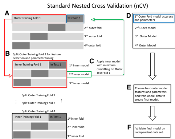
Fig. 1. Standard nCV. (A) Split the data into outer folds of training and testing data pairs (four outer folds in this illustration). Then do the following for each outer training fold {illustration starting with Outer Training Fold 1 [red box (A)]}. (B) Split outer training fold into inner folds for feature selection and possible hyperparameter tuning by grid search. (C) Use the best inner training model including features and parameters (second inner model, green box, for illustration) based on minimum overfitting (difference between training and test accuracies) in the inner folds to test on the outer test fold (green arrow to blue box, Test Fold 1). (D) Save the best model for this outer fold including the features and test accuracies. Repeat (B)–(D) for the remaining outer folds. (E) Choose the best outer model with its features based on minimum overfitting. Train on the full data to create the final model. (F) Validate the final model on independent data. (Color version of this figure is available at Bioinformatics online.)
