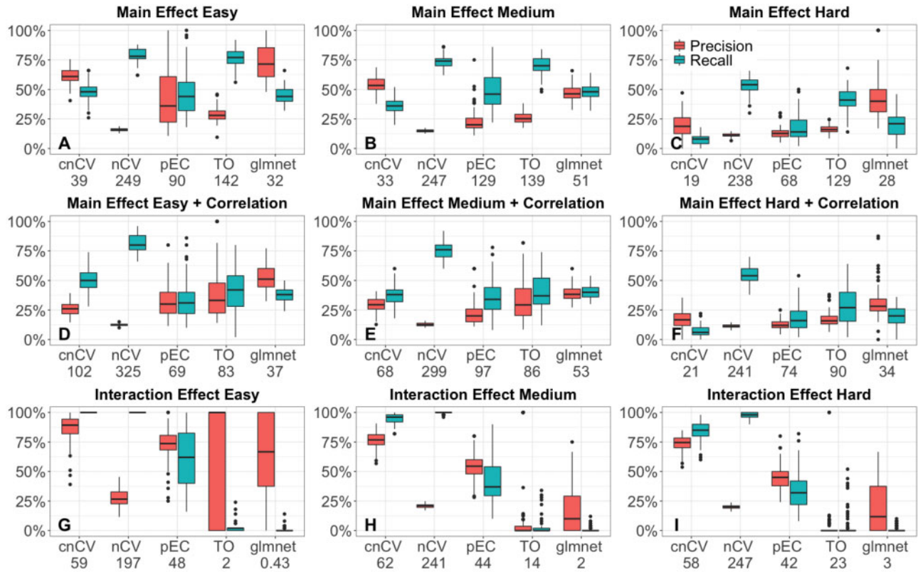
Fig. 4. Precision (red) and recall (teal) for selecting functional features (50 functional out of p=500 and m=200 samples) for cnCV, standard nCV, pEC, differential privacy TO and glmnet for 100 replicate simulated datasets with main effects (A–C), main effects with correlation (D–F) and interaction effects (G–I). Effect sizes range from easy to hard (left to right). The number below each method (on horizontal axes) is the average number of features selected by the method. Precision and recall computed from the training/holdout data. (Color version of this figure is available at Bioinformatics online.)
