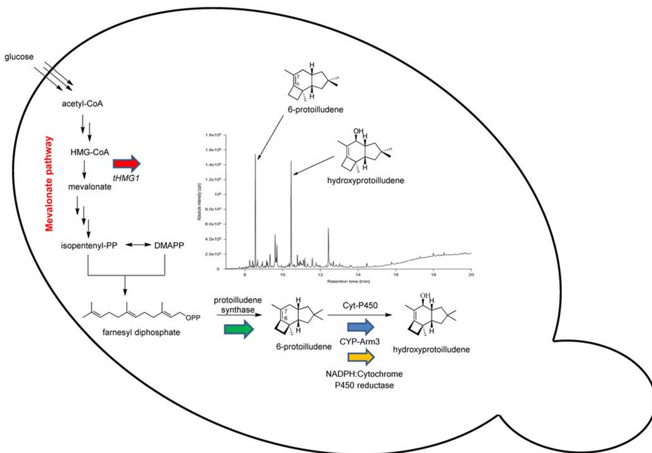
Fig. 7 The production of a novel hydroxyprotoilludene in Saccharomyces cerevisiae by metabolic engineering. The cells were engineered to overexpress the catalytic domain of 3-hydroxy-3-methylglutaryl-CoA-reductase (red arrow) to increase the production of
