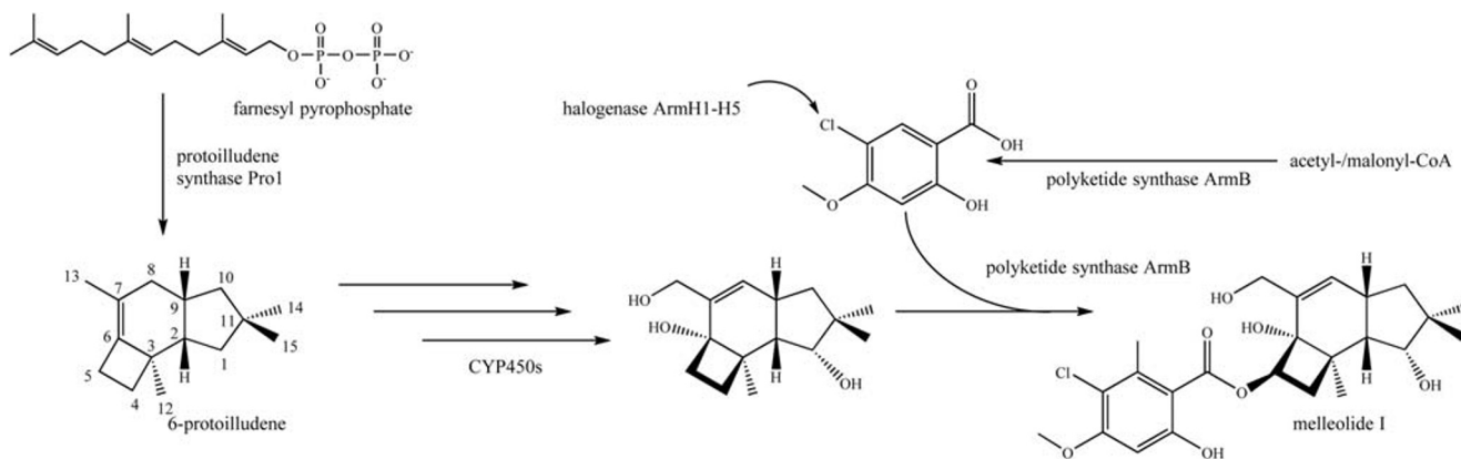
Fig. 2 The melleolide I biosynthesis pathway. The pathway begins with the cyclization of farnesyl diphosphate to 6-protoilludene (Engels et al. 2011) and then oxygenation catalyzed by cytochrome P450 monooxygenases. The final step is the attachment of an orsellinic acid, produced, and transferred by the polyketide synthase ArmB (Lackner et al. 2013). Subsequent chlorination of the side chain is carried out by
