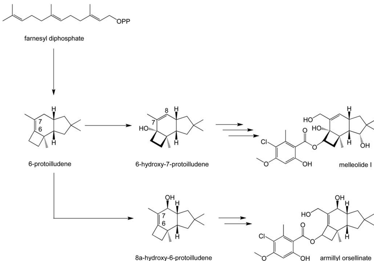
Fig. 8 The novel hydroxyprotoilludene was identified as 8 \alpha -hydroxy-6-protoilludene by NMR spectroscopy. This is the first step in the biosynthesis of melleolides with the carbon double bond in the 6,7 position (like
