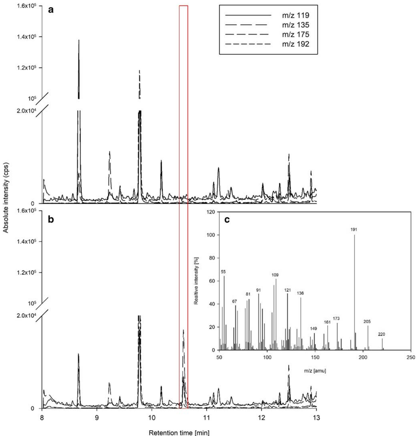
Fig. 6 Nonradioactive feeding assay and GC/MS analysis of extracts from cells supplemented with exogenous 6-protoilludene. GC/MS chromatogram and analysis by selective ion monitoring (SIM) based on literature values for the masses of 6-protoilludene (Joulain and König 1998) and 6-hydroxy-7-protoilludene (Nozoe et al. 1977). (A) Extract of negative control cells expressing TcCPR alone. (B) Extract from cells
