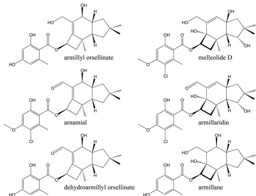
Fig. 1 Selected armillyl orsellinate and melleolide structures produced by Armillaria gallica FU02472. The structures differ in the presence/absence or position of the double bond in the six-ring system, the number and position of hydroxyl groups, and modifications of the orsellinic acid side chain such as halogenation
