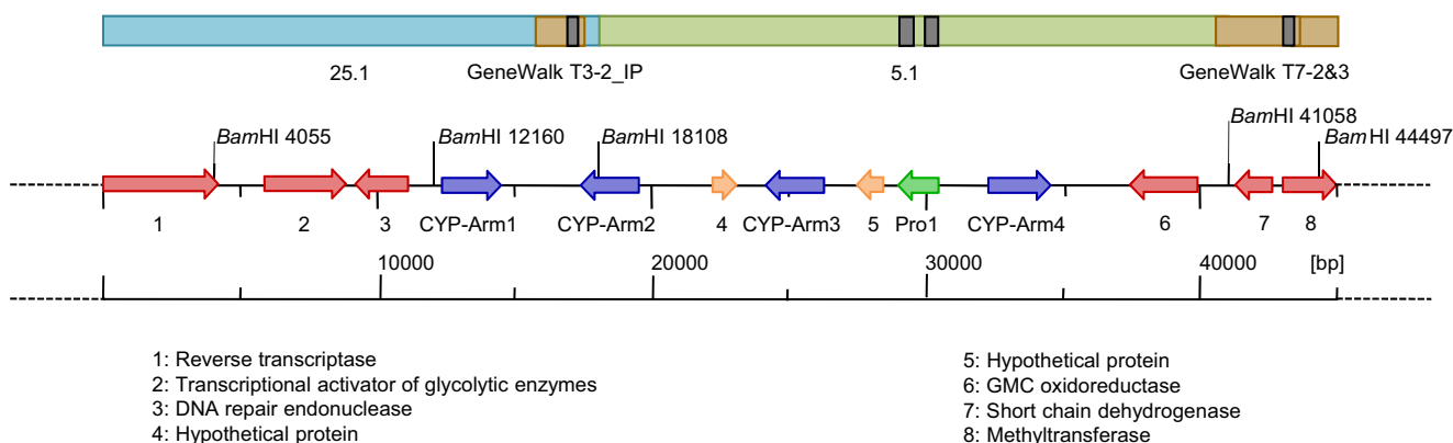
Fig. 3 Map of the melleolide gene cluster. Schematic representation of the terpene biosynthesis part of the melleolide gene cluster obtained by screening a genomic DNA library with probes matching the protoilludene synthase coding region and untranslated regions (black bars). The cluster contains the protoilludene synthase gene (green arrow), four genes
