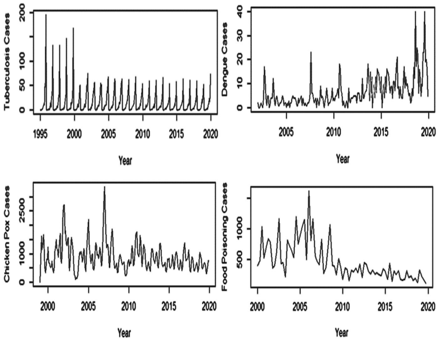
Fig. 2 Time series representation of disease datasets to demonstrate the trend and seasonality in the data
