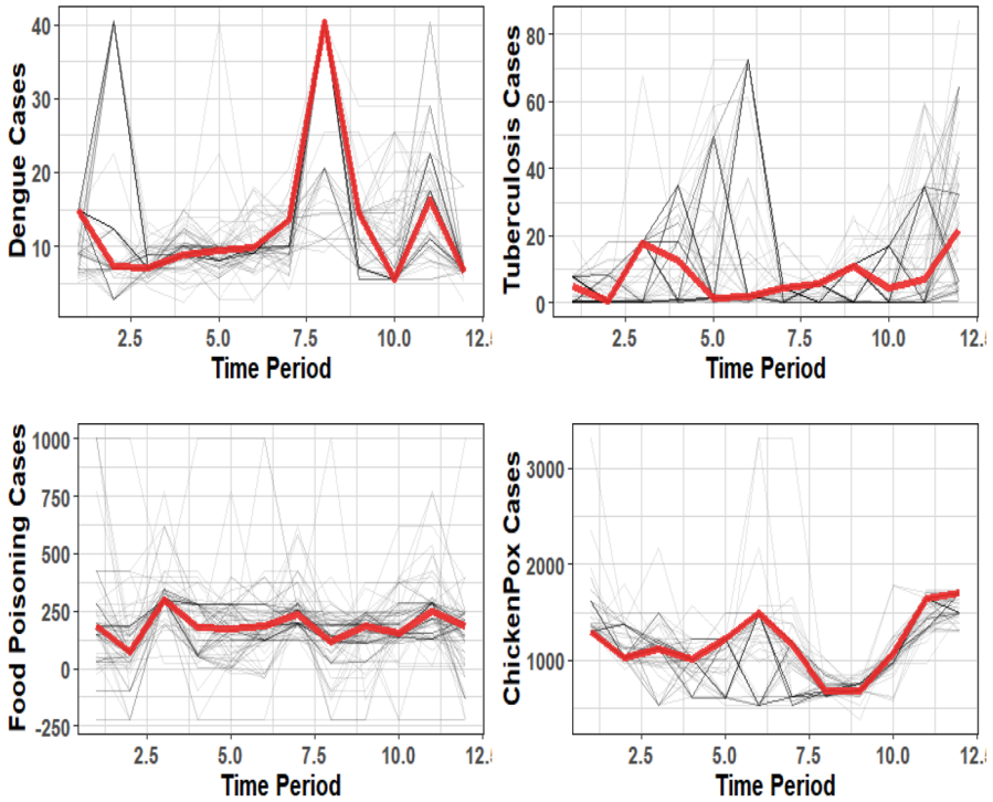
Fig. 3 Application of ensemble model on the bootstrapped datasets. Lighter grey lines represent the individual forecasts of the model. Red line represents the final forecast
