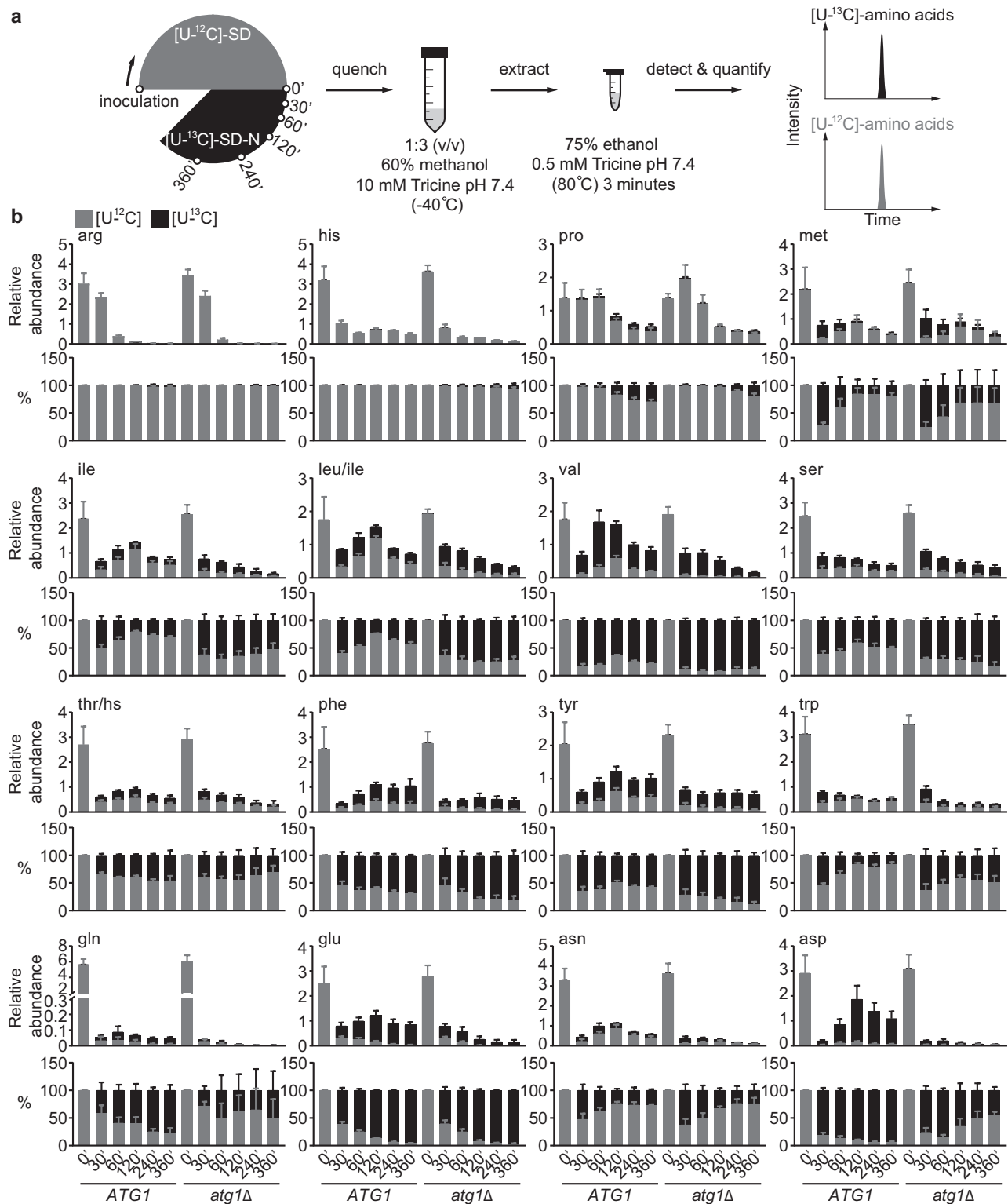
Fig. 2 Autophagy promotes the synthesis of specific amino acids under nitrogen starvation. a Schematic of the experimental design. WT ( ATG1 ) and atg1Δ cells were grown in SD and starved in [U-^{13}C] -SD-N for varying times. Metabolites were extracted and analyzed by LC-MS/MS. b Changes of [U-^{12}C] - and [U-^{13}C] -amino acids in nitrogen-starved WT and atg1Δ cells. Three independent replicates for leu/ile, five for his, nine for asp, and six for the remaining amino acids. WT and atg1Δ cells were always processed and analyzed together and therefore their relative abundances are directly comparable. hs: homoserine.
