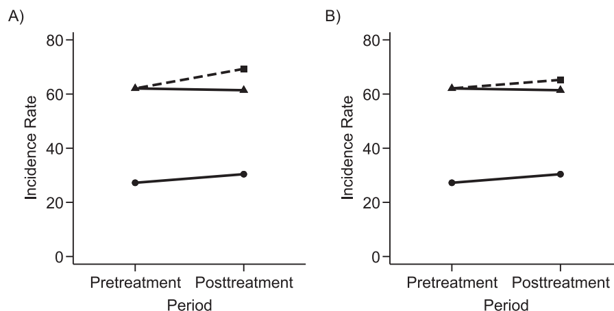
Figure 1. Graphical depiction of identification using the prior event rate ratio (PERR) and the prior event rate difference (PERD). Observed incidence rates, denoted by circles for the control group and triangles for the treated group (connected by solid lines to highlight the change between the pretreatment and the posttreatment periods), are identical in both panels. The observed incidence rate in the control group ( A = 0 ) increased from 27.24 in the pretreatment period to 30.41 in the posttreatment period. A) On the multiplicative scale, that is an increase by a factor of 1.12. Using PERR, the counterfactual posttreatment rate in the treated group is estimated to be the observed pretreatment rate, 62.07, increased by the same factor: 62.07 \times 1.12 = 69.29 (dashed lines highlight the change between the pretreatment rate and the counterfactual posttreatment rate). B) On the additive scale, the increase in the control group is 3.17. Using PERD, the counterfactual posttreatment rate in the treated group is estimated to be the observed pretreatment rate, 62.07, increased by 3.17, that is 62.07 + 3.17 = 65.24 . All rates are expressed as events per 1,000 person-years. Data for this illustration is from Table 4 in Othman et al. (5).
