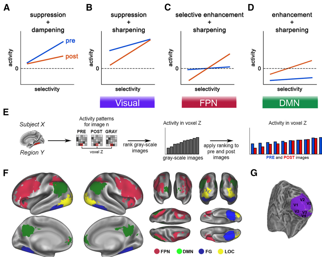
Figure 1. A–D , Alternative explanatory mechanisms of prior-induced changes in neural activity. E , Schematic for the image preference analysis. For each voxel within an ROI, images are ranked based on the activation magnitudes in the grayscale condition. This image ranking is then applied to the same voxel's activity during pre- and post-disambiguation conditions (for details, see Image preference analysis). F , Locations of FPN and DMN ROIs (red and green), and category-selective visual areas (FG and LOC, blue and yellow). G , Location of early visual areas in an example subject.
