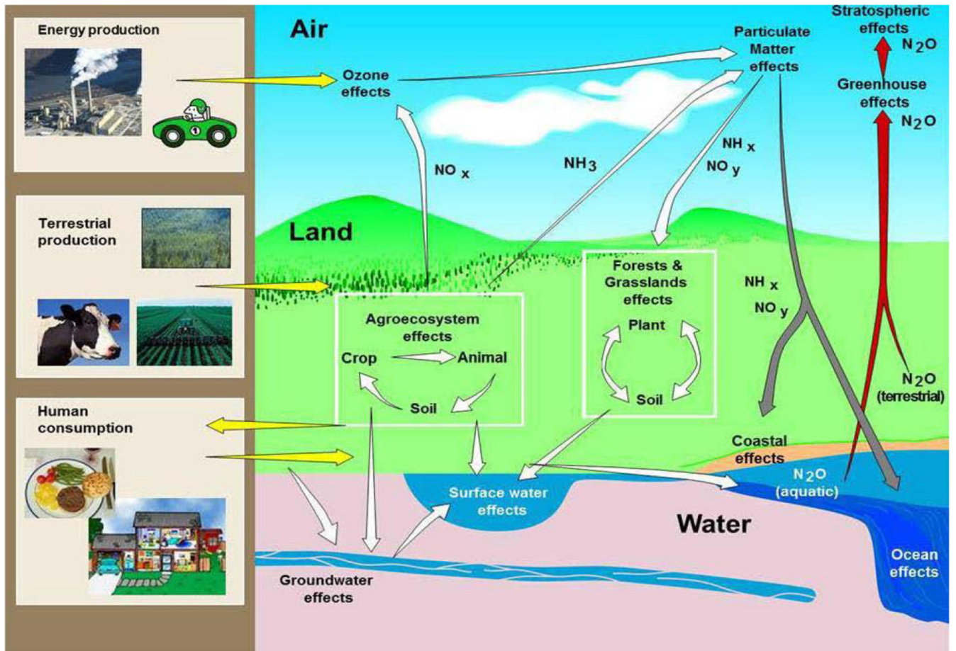
Figure 1: The nitrogen cascade (Source: [60], adapted from [61]).
