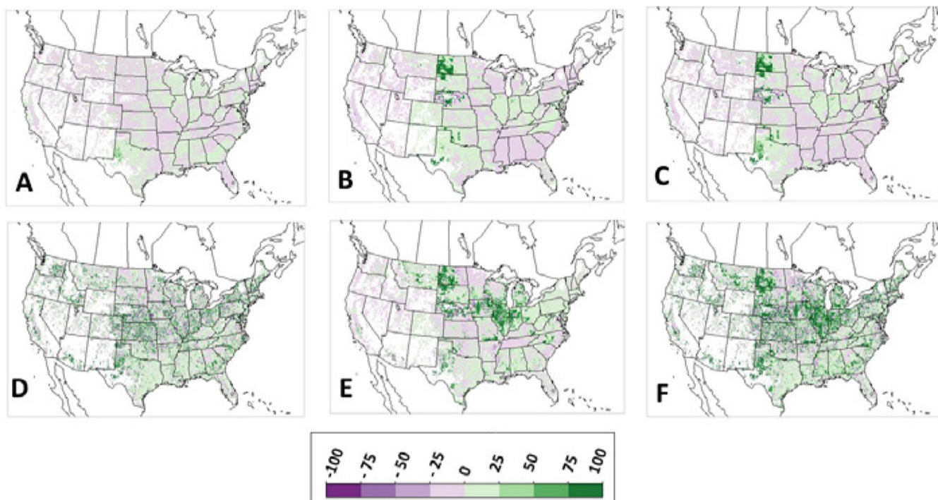
Figure 6: Percent change (%) from 2002 conditions for surface runoff attributable to A) trends only (Equation. 1), B) stover removal and cropland reallocation only (Equation. 2), C) all factors (Equation. 3), and N export attributable to D) trends only (Equation. 1), E) stover removal and cropland reallocation only (Equation. 2), and F) all factors (Equation. 3). N export includes dissolved inorganic N losses in surface and sub-surface lateral flow. Purple represents a decrease and green represents an increase. Unity values, i.e. no change are included in the lightest green bin.
