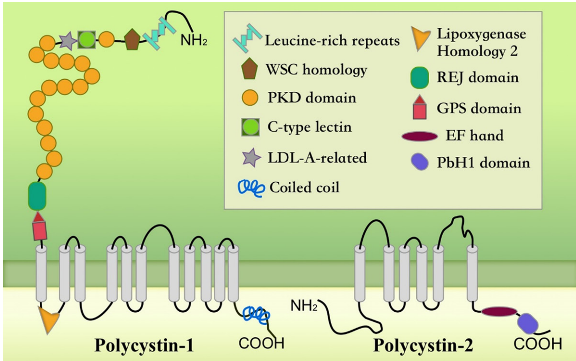
Figure 4. Structure of polycystins. PC1 has a large extracellular domain, 11-transmembrane domain, and short C tail. PC2 has a six-transmembrane domain and cytoplasmic N- and C-termini. The coiled-coil domain in the C-terminal end of PC1 interacts with the C-terminal tail of PC2.
