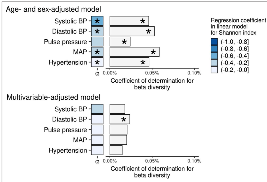
Figure 1. Associations between blood pressure (BP) variables and microbial diversity. The blue heat maps on the left express the change in BP variables per 1-SD increase in \alpha diversity (Shannon index); log odds are reported for hypertension. The bar plots on the right represent the proportion of variability ( R^2 ) in \beta diversity (Bray-Curtis distance) explained by BP indexes. Multivariable-adjusted model is adjusted for age, sex, body mass index, smoking, exercise, diuretics, \beta blockers, calcium channel blockers, and renin-angiotensin system blockers. Significant results are marked with asterisk ( P < 0.05 ). \alpha indicates effect size for \alpha diversity; and MAP, mean arterial pressure.
