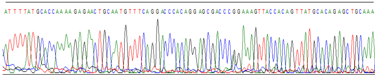
Figure 1. Sequence analysis of the HPV16 E6 region. Sequences for the HPV16 E6 region were investigated using PCR products in HPV16 DNA positive cases. HPV16, human papillomavirus type 16.
