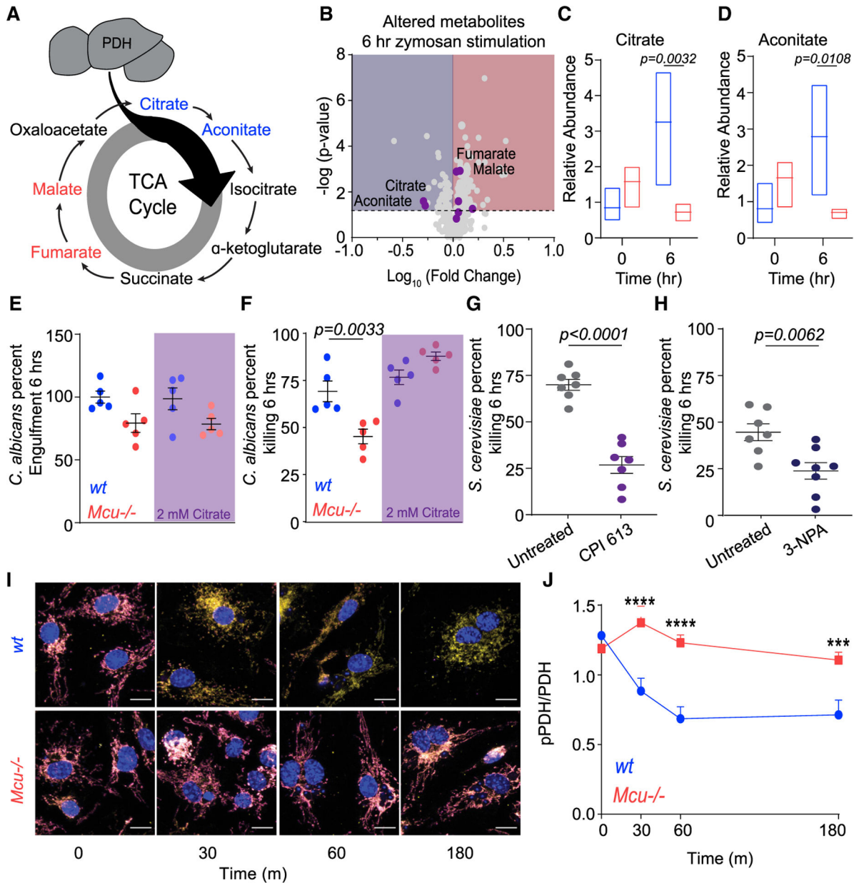
Figure 7. Dysregulated TCA Cycle Underlies Defective Killing by Mcu -/- Macrophages (A) Schematic of TCA cycle. Metabolites reduced in Mcu -/- BMDMs responding to zymosan (6 h) are blue. Metabolites that increased in Mcu -/- BMDMs are red. (B) Volcano plot of significantly altered metabolites in Mcu -/- macrophages compared to WT following 6 h of zymosan stimulation. The dotted horizontal line represents the 75th percentile for -\log(p\text{-value}) . TCA cycle metabolites are shown as purple dots. (C) Relative abundance of citrate measured in WT (blue) and Mcu -/- (red) BMDMs at baseline and 6 h following zymosan stimulation. Floating bars represent the minimum to maximum, and the line is at the mean for each dataset; p = 0.0032 was detected according to two-way ANOVA, two tailed.
