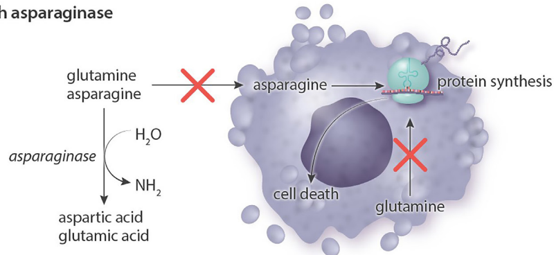
Figure 3. Mechanism of action of asparaginase. The lack of asparagine synthetase in NK/T-cells means that they are dependent on exogenous asparagine and glutamine. By degrading asparagine and glutamine to aspartic acid and glutamic acid, asparaginase inhibits essential intracellular protein synthesis and triggers cell death. NK = natural killer.
