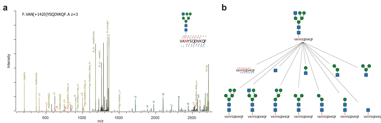
Figure 9. Hybrid EThcD fragmentation yields rich structural data on viral glycopeptides. (a) EThcD MS/MS spectrum of a glycopeptide derived from the MERS-CoV S protein as described in ref 116. A multitude of b/c/y/z-ions originating from peptide backbone fragmentation are detected and enable accurate site localization. In addition fragments of the glycan, conjugated to the peptide, are observed as well as oxonium signature fragment ions, all in one MS/MS spectrum. (b) Overview of the assigned fragments in the EThcD spectrum of panel a, enabling structural reconstruction of the glycopeptide.
