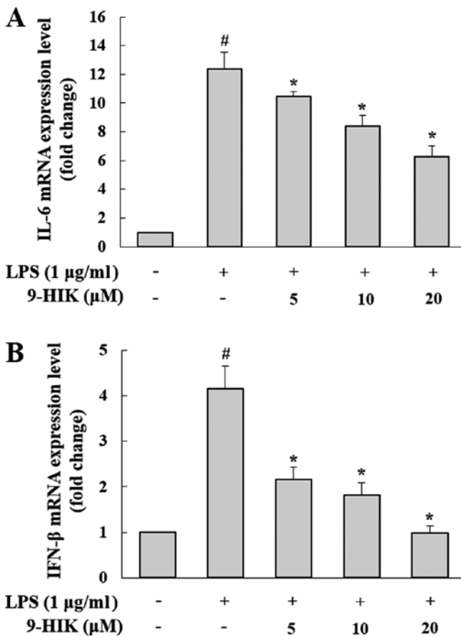
Figure 3. Effect of 9-HIK on IL-6 and IFN- \beta mRNA expression in LPS-stimulated RAW264.7 cells. RAW264.7 cells were pre-treated with various concentrations of 9-HIK for 2 h, then stimulated with LPS for 4 h. (A) IL-6 and (B) IFN- \beta mRNA expression levels. Data are presented as the mean \pm SD; n=3. # P<0.05 vs. control; * P<0.05 vs. LPS-treated cells. 9-HIK, 9-hydroxy-isoegomaketone; IFN- \beta , interferon- \beta ; LPS, lipopolysaccharide.
