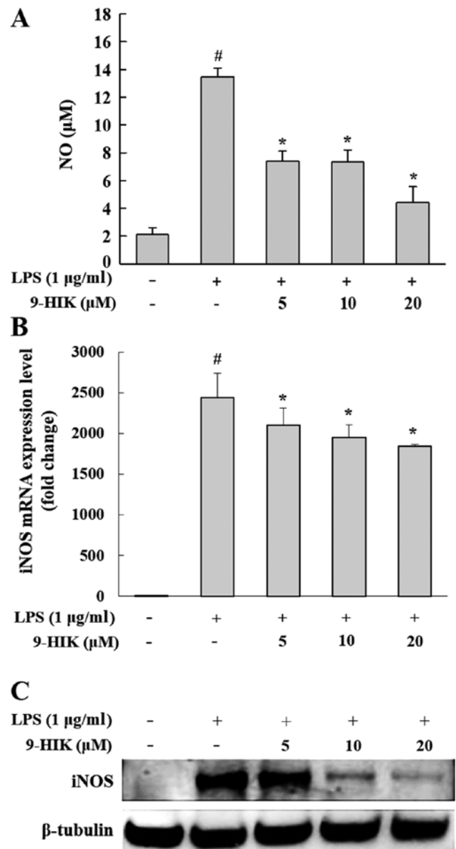
Figure 2. Effects of 9-HIK on NO production and iNOS expression in LPS-treated RAW264.7 cells. RAW264.7 cells were pre-treated with various concentrations of 9-HIK for 2 h, then stimulated with LPS for 18 h. (A) NO production. (B) iNOS mRNA expression levels. (C) iNOS protein expression levels. Data are presented as the mean \pm SD; n=3. #P<0.05 vs. control; *P<0.05 vs. LPS-treated cells. 9-HIK, 9-hydroxy-isoegomaketone; LPS, lipopolysaccharide; iNOS, inducible nitric oxide synthase; NO, nitric oxide.
