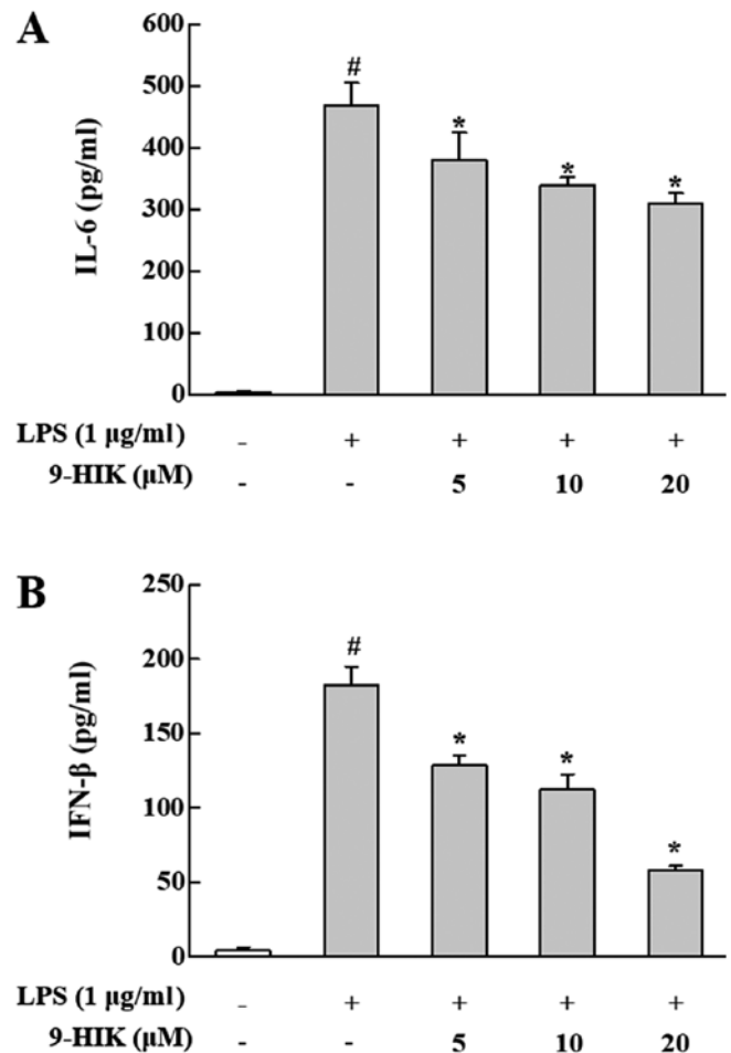
Figure 4. Effect of 9-HIK on IL-6 and IFN- \beta protein expression in LPS-stimulated RAW264.7 cells. RAW264.7 cells were pre-treated with various concentrations of 9-HIK for 2 h, then stimulated with LPS for 4 h. (A) IL-6 and (B) IFN- \beta protein expression levels. Data are presented as the mean \pm SD; n=3. # P<0.05 vs. control; * P<0.05 vs. LPS-treated cells. 9-HIK, 9-hydroxy-isoegomaketone; IFN- \beta , interferon- \beta ; LPS, lipopolysaccharide.
