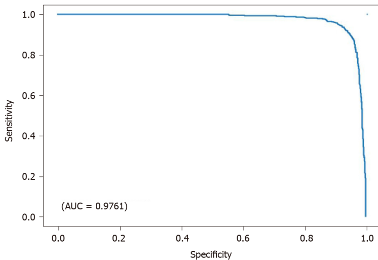
Figure 2 Receiver operating characteristic curve for the test dataset. The area under the curve (AUC) was above 97%.
