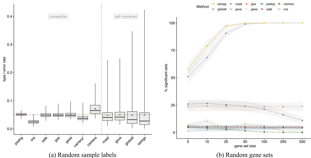
Figure 4. Random sample labels and random gene sets. (a) Type I error rates (y-axis) as evaluated on the dataset from Golub et al. [42] by shuffling sample labels 1000 times and assessing in each permutation the fraction of gene sets with P < 0.05 . Gene sets were defined according to GO-BP ( N = 4631 ). Blue points indicate the mean type I error rate and the red dashed line the significance level of 0.05. The gray dashed line divides methods based on the type of null hypothesis tested [6]. *Application of CAMERA without accounting for inter-gene correlation (default: inter-gene correlation of 0.01). Supplementary Figure S5 shows type I error rates when using KEGG gene sets. Supplementary Figure S6 shows type I error rates for all four combinations of benchmark compendium and gene set collection. (b) Percentage of significant gene sets ( P < 0.05 , y-axis) when applying methods to the Golub dataset (true sample labels) and using 100 randomly sampled gene sets of defined size (x-axis). Shown is the mean \pm standard deviation (gray bands) across 100 replications of the simulation experiment.
