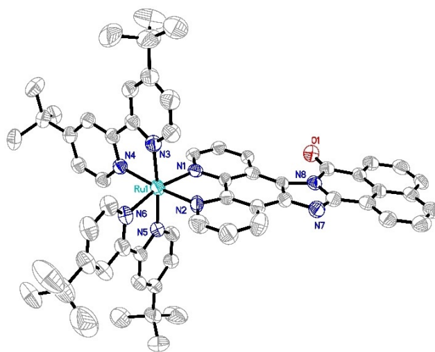
Figure 3. Solid-state structure (ORTEP representation) of Rubiipo with thermal ellipsoids at a probability level of 50%. Hydrogen atoms, PF 6 - counterions and solvent molecules are omitted for clarity. Deposition number 1993565 ( Rubiipo ) contains the supplementary crystallographic data for this paper. These data are provided free of charge by the joint Cambridge Crystallographic Data Centre and Fachinformationszentrum Karlsruhe Access Structures service.
