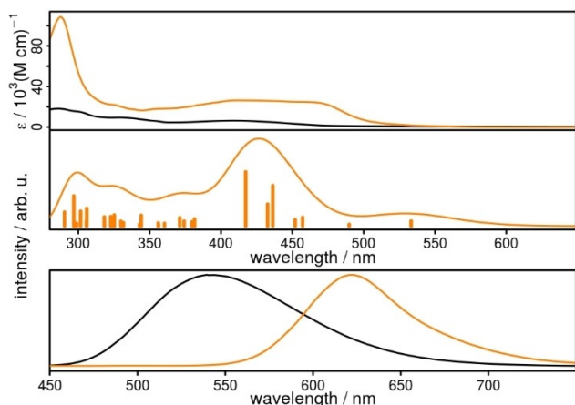
Figure 5. Spectra of biipo (black) and Rubiipo (orange). Top) UV/Vis absorption spectrum in acetonitrile. Middle) Calculated absorption spectrum of Rubiipo resulting from the convolution (std. deviation 40) of the transitions above 290 nm (vertical bars) with a Gaussian function. The transition energies are calculated at full TD-DFT level of theory (B3LYP-D3(BJ)/def2-TZVP. Bottom) Emission spectra in acetonitrile under oxygen-free conditions.
