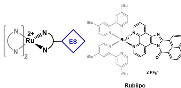
Figure 1. Schematic representation of a Ru II photosensitizer containing an additional electron storage (ES) moiety (left) and the structure of Rubiipo investigated in this study (right). The biipo ligand is depicted in black.
