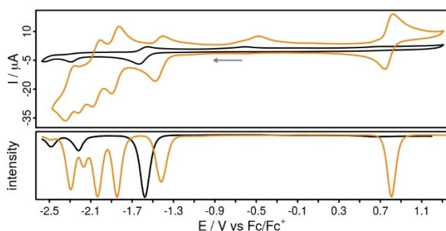
Figure 4. Cyclic voltammograms (top) and differential pulse voltammograms (DPV, bottom) of biipo (black, concentration < 1 mM due to low solubility in acetonitrile) and Rubiipo (orange, 1 mM) in acetonitrile solution referenced vs. the ferrocene/ferricenium ( \text{Fc}/\text{Fc}^+ ) couple. The current values of the DPV are normalized. Conditions: scan rate of 100 \text{ mV s}^{-1} , [\text{Bu}_4\text{N}][\text{PF}_6] (0.1 M) as supporting electrolyte.
