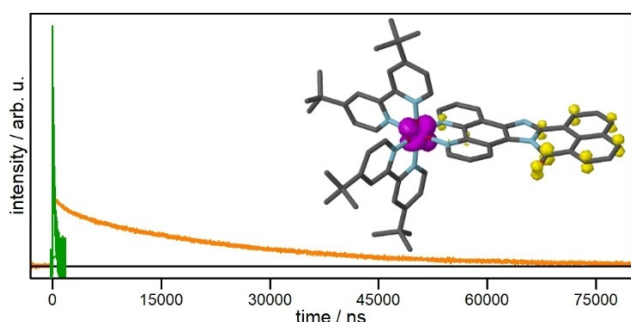
Figure 6. Emission lifetime of Rubiipo in acetonitrile under ambient (green) and inert conditions (orange). The respective fits and the residuals are depicted in the Supporting Information. The inset (differential density plot of Rubiipo ) shows one of the occurring MLCT transitions from the ruthenium d orbital to the \pi^* orbital located at the naphthaloylenebenzene moiety.
