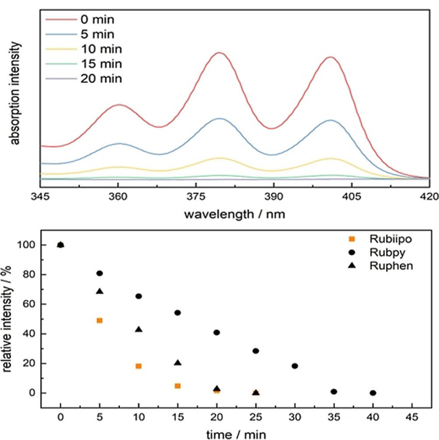
Figure 8. Top) Singlet oxygen evolution experiment using Rubiipo (1 equiv.) and ABDA (50 equiv.) in PBS after irradiation with blue light ( 50\ \text{mWcm}^{-2} , 470 nm) in the range of ABDA absorbance (see also Figure S4.5). Bottom) Comparison of the relative ABDA absorbance as function of time during irradiation of Rubiipo (squares), Rubpy (circles) and Ruphen (triangles) with blue light ( 50\ \text{mWcm}^{-2} , 470 nm). It becomes clear, that Rubiipo degrades ABDA the fastest. See for the specific ABDA test in the Supporting Information the section 4.
