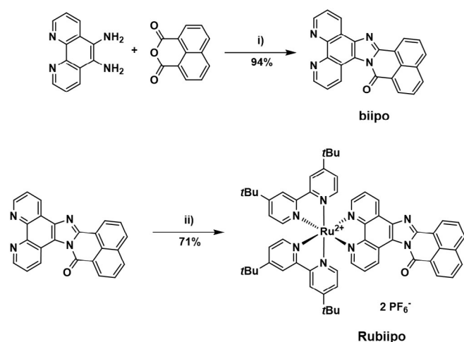
Figure 2. Preparation of the biipo ligand and its corresponding Ru II complex Rubiipo . Conditions: i) acetic acid, Ar, 140 °C, 24 h and ii) [(\text{tbbpy})_2\text{RuCl}_2] , ethylene glycol, 120 °C, 20 h.
