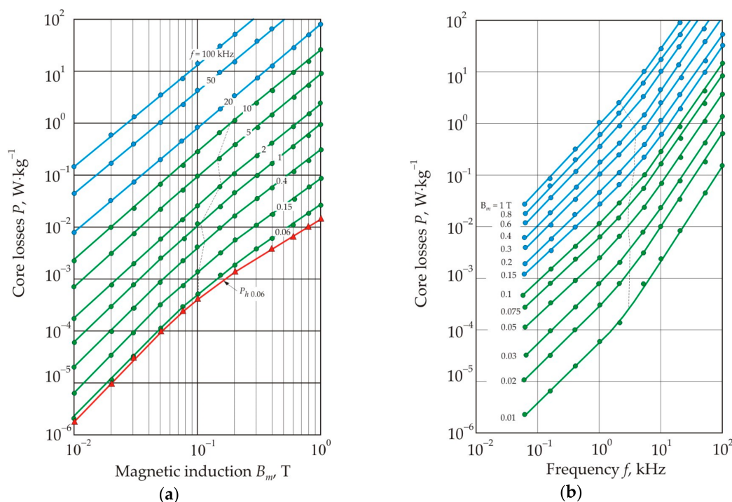
Figure 30. Dependences of core losses P on magnetic induction B_m at different frequency f (a) and dependences of core losses P on frequency f for different magnetic induction B_m in the Fe_{72.5}Cu_1Nb_2Mo_{1.5}Si_1 alloy after heat treatment without a magnetic field. The numbers on the curves indicate the frequency f in kHz (a) and the magnetic induction B_m in T (b). Curve Ph_{60} corresponds to hysteresis losses at a frequency of 60 Hz. The dashed line marks the transition points that correspond to the change in the slope of the linear sections of the curves. Reproduced with permission from [94].
