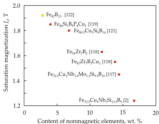
Figure 25. Dependence of saturation magnetization J_s on the mass content of non-magnetic elements in nanocrystalline soft magnetic alloys with a coercive force less than 6 \text{ A}\cdot\text{m}^{-1} . The \text{Fe}_{87}\text{B}_{13} alloy was obtained at a heating rate of 3 \text{ K}\cdot\text{s}^{-1} .
