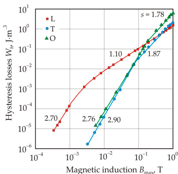
Figure 27. Dependences of hysteresis losses W_h on the maximum induction B_{\max} after heat treatment in a longitudinal (L) and transverse (T) magnetic field, as well as without a magnetic field (O), for cores made of nanocrystalline \text{Fe}_{67.5}\text{Co}_5\text{Cu}_1\text{Nb}_2\text{Mo}_{1.5}\text{Si}_{14}\text{B}_9 alloy. The numbers on the curves represent the exponent s for the power function (25). Reproduced with permission from [100].
