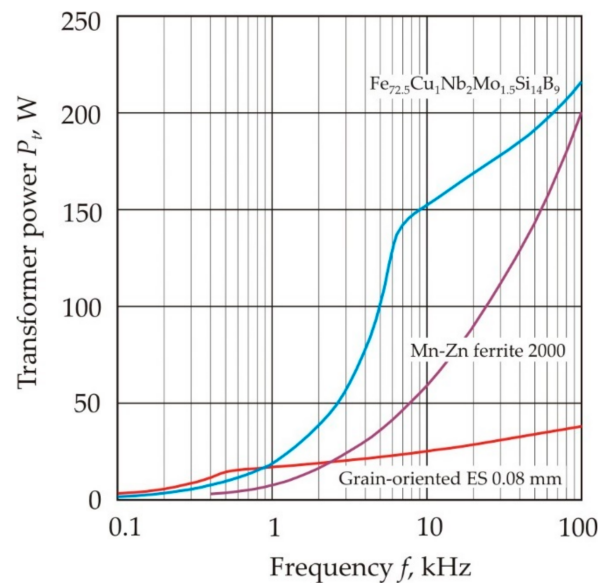
Figure 35. Power of transformers P_t as a function of frequency f for a magnetic core made of different soft magnetic materials, which has an outer diameter of 20 mm, an inner diameter of 32 mm and a height of 10 mm. Adapted from [139].
