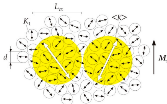
Figure 1. Schematic representation of the magnetic structure of a nanocrystalline soft magnetic alloy. Adapted from [15].
