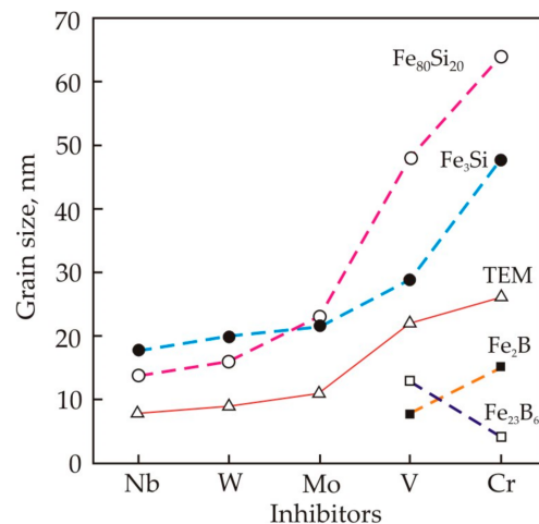
Figure 16. Average grain size from transmission electron microscopy (TEM) and average size of crystalline phases \text{Fe}_{80}\text{Si}_{20} , \text{Fe}_3\text{Si} , \text{Fe}_2\text{B} , and \text{Fe}_{23}\text{B}_6 from X-ray analysis in \text{Fe}_{73.5}\text{Cu}_1\text{M}_3\text{Si}_{13.5}\text{B}_9 alloys with inhibitors M = \text{Nb}, \text{W}, \text{Mo}, \text{V}, \text{Cr} . Reproduced with permission from [77].
