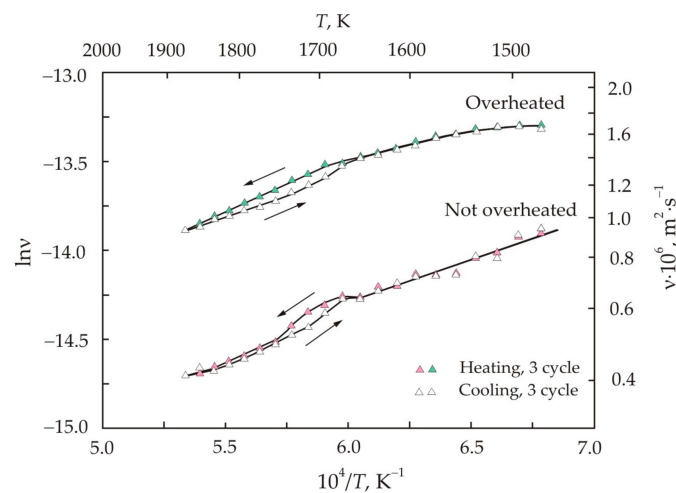
Figure 7. Temperature dependences of kinematic viscosity \nu for the third heating—cooling cycle in the overheated and not overheated melt prepared from the amorphous \text{Fe}_{72.5}\text{Cu}_1\text{Nb}_2\text{Mo}_{1.5}\text{Si}_{14}\text{B}_9 ribbon. The arrows show the direction of temperature change [45].
