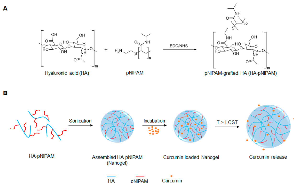
Figure 1. Schematic representation of (A) the preparation of pNIPAM-grafted hyaluronic acid (HA-pNIPAM) and (B) the assembly of HA-g-pN nanogel and curcumin release.
