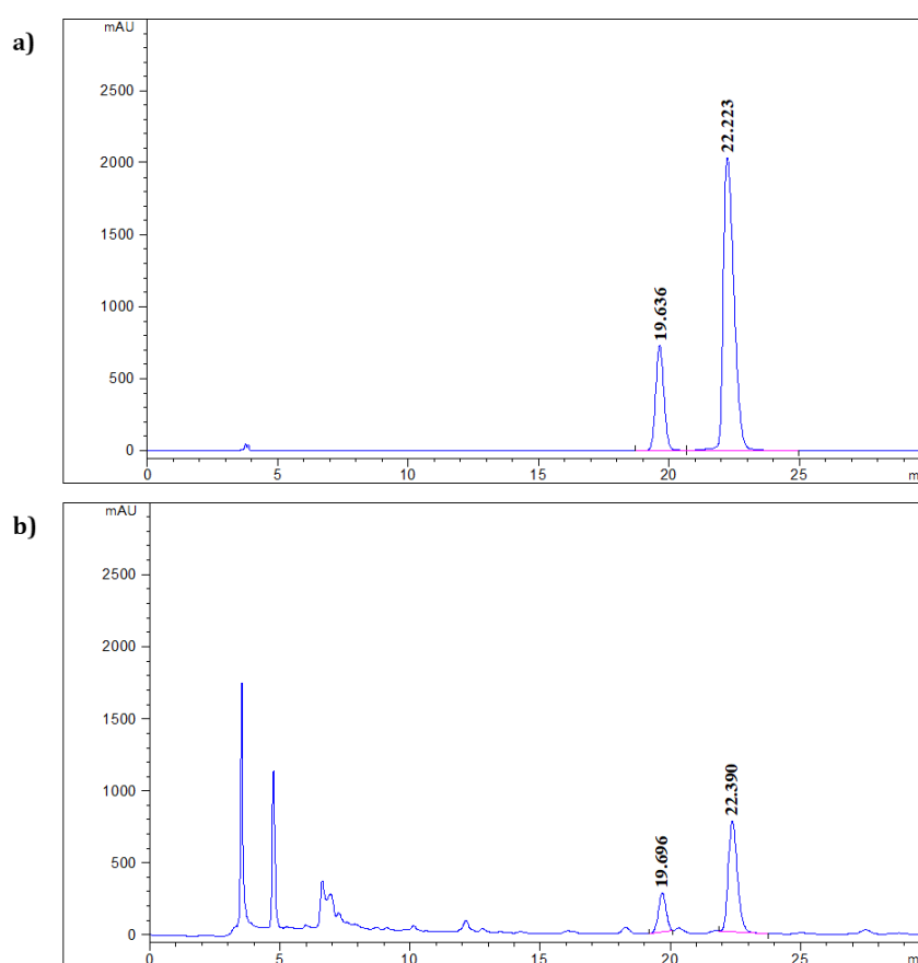
Figure 2. HPLC chromatogram of (a) mixed standard of quercetin-3- O -glucuronide (19 min) and ellagic acid (22 min), and (b) ethanol extract of O. biennis sprout.
