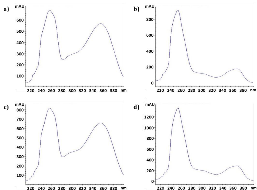
Figure 3. UV spectrum structure of quercetin-3- O -glucuronide and ellagic acid. (a) Quercetin-3- O -glucuronide reference; (b) Ellagic acid reference; (c,d) O. biennis sprout ethanol extract.
