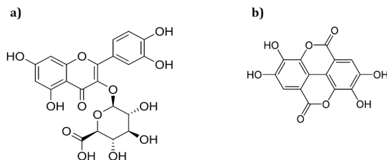
Figure 1. Chemical structure of (a) quercetin-3- O -glucuronide and (b) ellagic acid.
