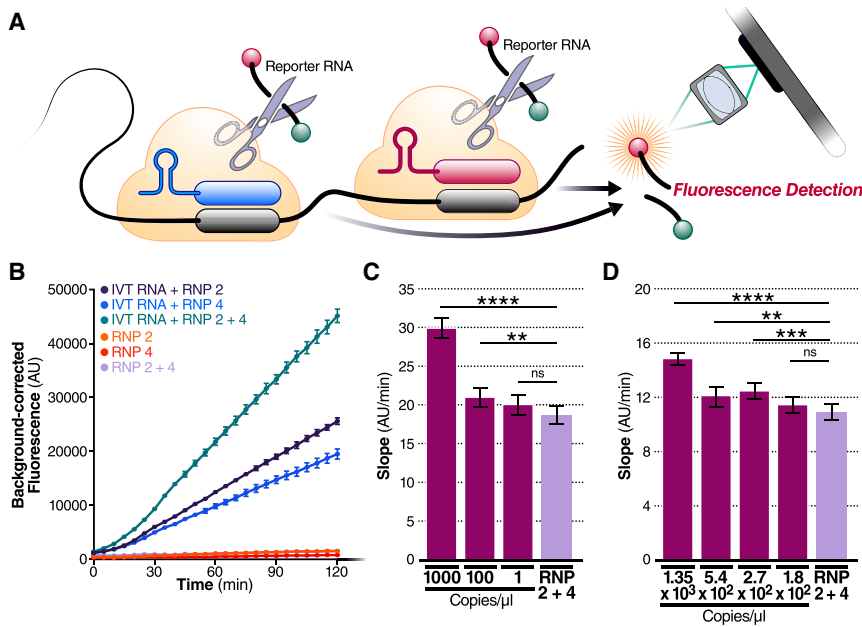
Figure 2. Combining crRNAs improves sensitivity of Cas13a
