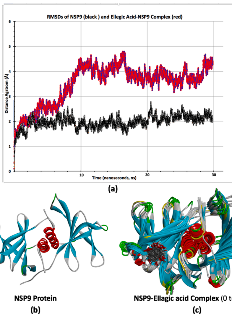
Fig. 9. RMSDs of nsp9 (black color) and Ellagic acid-nsp9 complex (red color) (a), the apo-form of nsp9 crystal structure (b), different structural frames of nsp9-Ellagic acid complex from 0 to 30 ns MD simulations.
