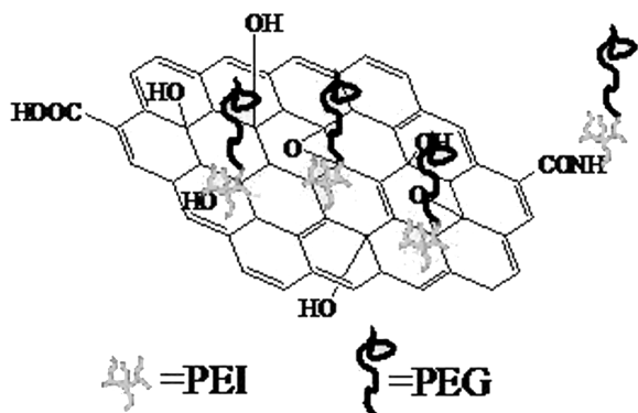
Figure 1. Structure of GO-PEI-PEG.
