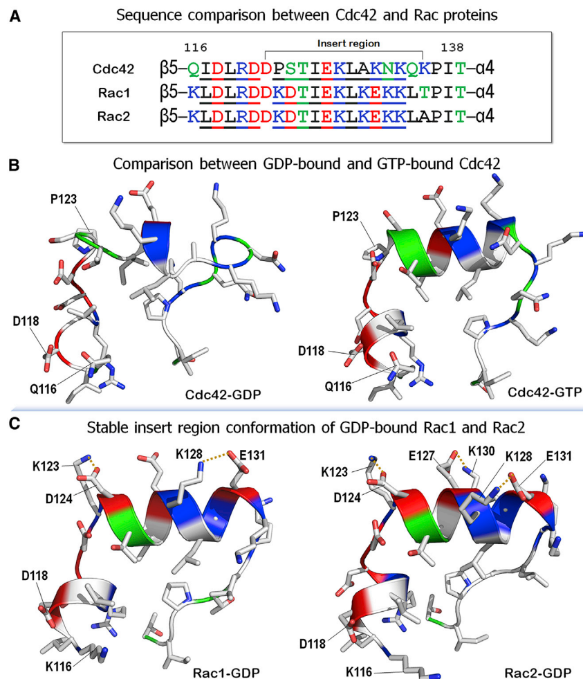
FIGURE 8 Comparison between Cdc42 and Rac1/Rac2 proteins. (A) Sequences of the insert region and its adjacent regions for Cdc42, Rac1, and Rac2. In the sequence, hydrophobic, polar/glycine, positively charged, and negatively charged residues are colored black, green, blue, and red, respectively. Underlining denotes the residues presenting the \alpha -helical structure. The former is the helix-forming 117 xDLRx 121 motif, and the latter is the insert region. Snapshots representing the final structures of insert region for (B) GDP-bound (left panel) and GTP-bound (right panel) Cdc42 and (C) Rac1-GDP (left panel) and Rac2-GDP (right panel) are shown. Rac proteins preserved a highly stable insert region during a 1- \mu s simulation. In the structures, colors are the same as in the sequence, except for the hydrophobic residues with white. Dotted lines denote salt bridges. To see this figure in color, go online.
