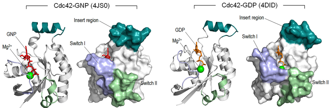
FIGURE 1 The sequence of Cdc42 aligned with the sequence of K-Ras4B (top panel). The crystal structures of GNP-bound (PDB: 4JS0) and GDP-bound (PDB: 4DID) Cdc42 are shown (bottom panel). Although the sequence and most structural motifs are highly conserved, K-Ras4B is missing the insert region (residues 122–135), an \alpha -helix rich in charged amino acids, which only appears in members of the Rho family. To see this figure in color, go online.
