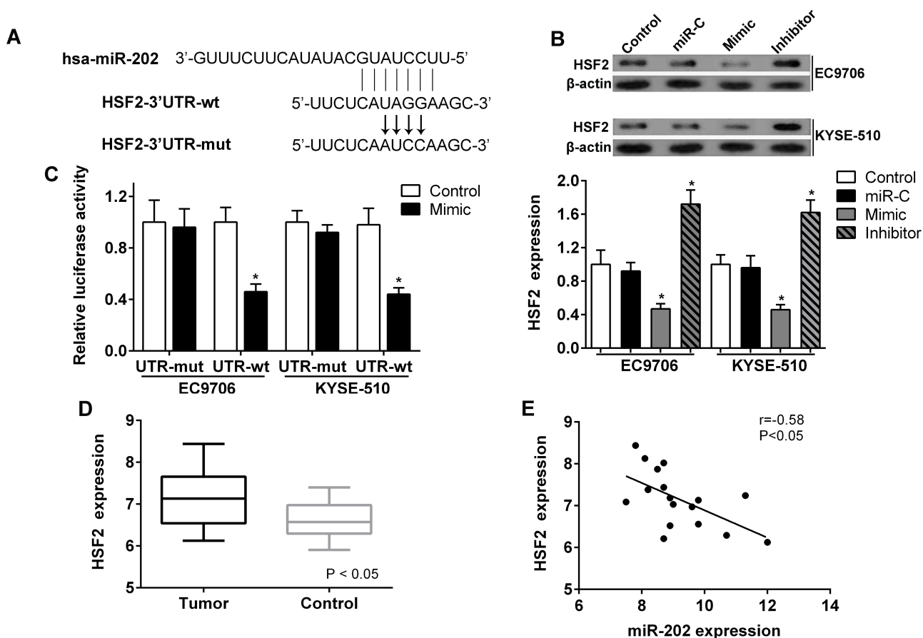
Figure 3. miR-202 directly targets the HSF2 mRNA. (A) miR-202 target sequences in the 3'-UTR of HSF2 mRNA predicted by searching the TargetScan and miRDB databases. (B) The protein expression of HSF2 in EC9706 and KYSE-510 cells was evaluated by Western blotting. (C) Luciferase activity was measured in cells transfected with HSF2-3'-UTR-wt (UTR-wt) or HSF2-3'-UTR-mut (UTR-mut). (D) Expression of HSF2 in human ESCC tumor tissue and adjacent noncancerous tissues (Control) of patients from the GEO database. (E) Correlation between HSF2 and miR-202 expression in ESCC tumor tissues (* p < 0.05 vs. Control).
