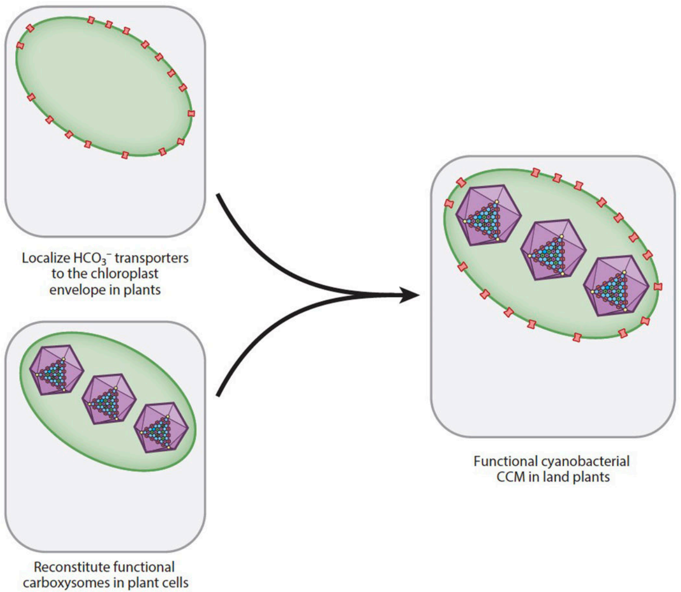
Figure 4. The goals of localizing HCO 3 - transporters to the proper plant membranes and building a carboxysome have been pursued in parallel. Once HCO 3 - transporters and carboxysomes can independently function in a plant cell, combining them into a single plant will be the next step toward reconstituting a cyanobacterial CO 2 concentrating mechanism (CCM) in land plants.
