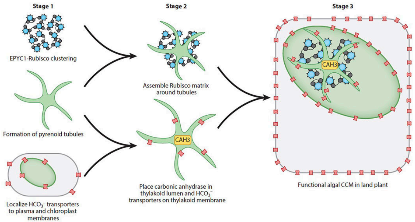
Figure 7. Several milestones toward engineering an algal CO 2 concentrating mechanism (CCM) into land plants can be pursued in parallel.
