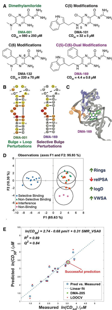
Figure 2. Dimethylamiloride (DMA) as a tunable RNA-binding scaffold.
