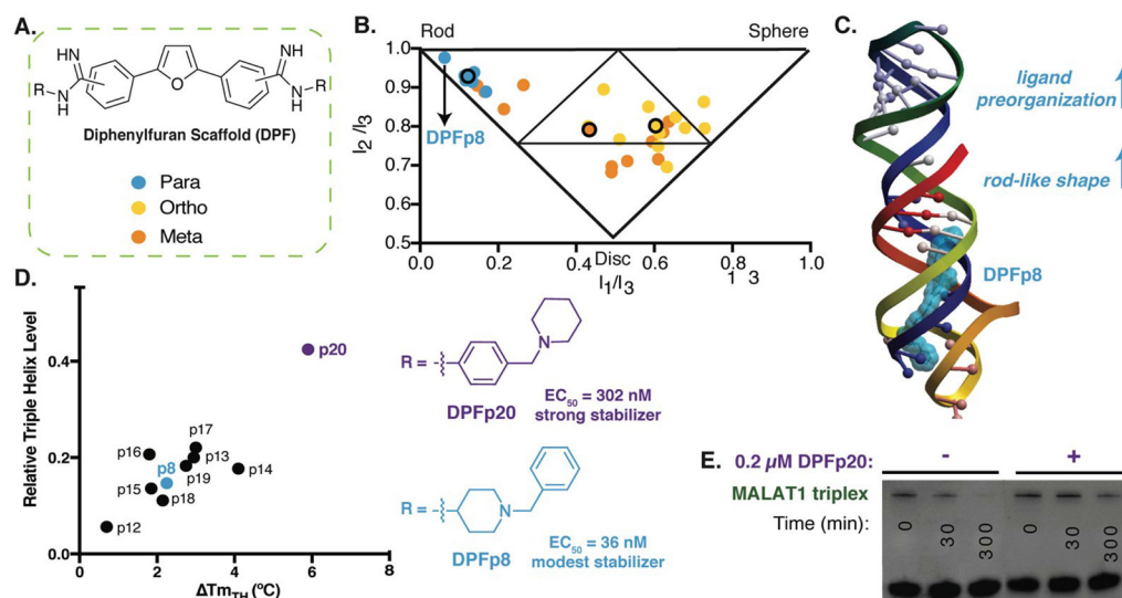
Figure 3. Diphenylfuran scaffold reveals shape-dependent RNA recognition of MALAT1 triplex. A. Schematic of diphenylfuran (DPF) scaffold library with symmetric regio-substitution. B. Principle moments of inertia (PMI) analysis of DPF library (blue-para, orange-meta, yellow-ortho substituted) revealed a correlation between triple helix binding strengths and small molecule 3D shape, with the highest affinity triplex binder (DPFp8) as the most rod-like. Reproduced from Ref. 94 with permission from John Wiley and Sons. C. Docking model of MALAT1 triple helix structure (PDB: 4PLX, Ref. 98) with DPFp8 (blue) illustrating the importance of rod-like shape and preorganization. D) Left: Correlation of DPF-induced changes in triplex melting temperature with amount of RNA remaining in an enzyme (RNaseR) degradation assay. Right: Structures of DPFp20, the most stabilizing DPF (purple) and DPFp8, the highest affinity DPF (blue). Shown EC_{50} values are based on RNA titration of fluorescent DPF scaffold. E. Gel image showing stabilization of MALAT1 triplex by DPF20 to RNaseR degradation. Panels D,E reproduced from Ref. 95 with permission from Oxford University Press.
