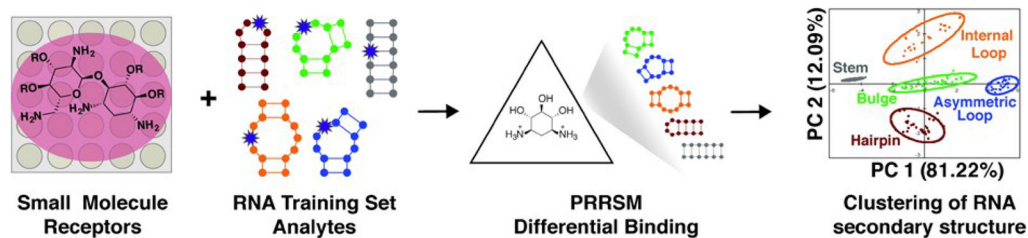
Figure 5: Pattern recognition of RNA by small molecules (PRRSM).
