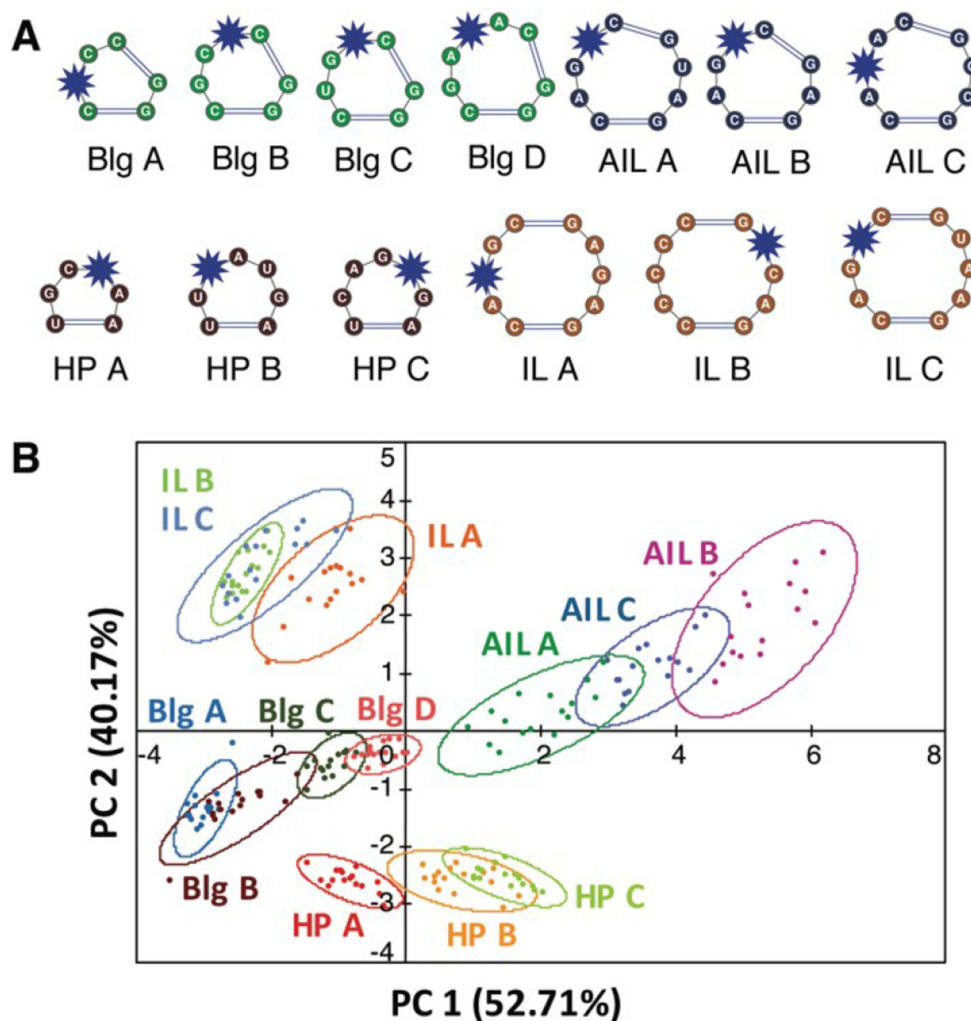
Figure 6. PRRSM classifies individual RNA secondary structures under dynamic conditions. A. Schematic of secondary structures (unpaired regions) in PRRSM RNA training set with BFU-labeled sites noted with a blue star. Reprinted with permission from Ref. 109. Copyright 2017 American Chemical Society. B. PCA plot of training set under conditions including polyethylene glycol (PEG) and increased temperature. Open ovals indicate 95% confidence intervals. The predictive power for the sequences was 92%. Buffer: 10 mM \text{NaH}_2\text{PO}_4 , 25 mM NaCl, 4 mM \text{MgCl}_2 , 0.5 mM EDTA, 8 mM PEG 12 000, pH 7.4 at 37 °C. Reproduced from Ref. 111 with permission from the Royal Society of Chemistry.
