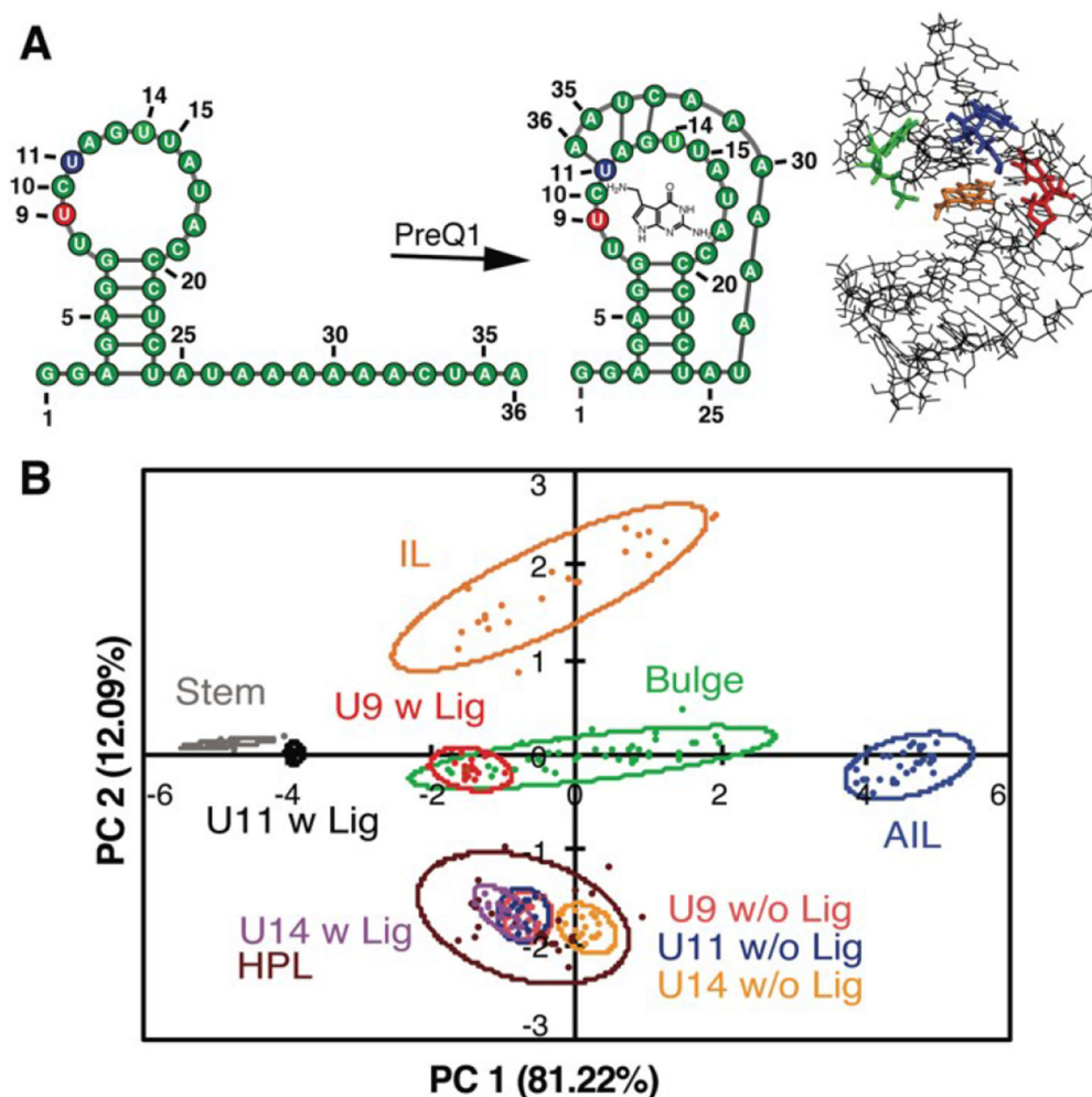
Figure 7. PRRSM classifies apo and bound secondary structures in prequeosine-1 (PreQ1) riboswitch.
