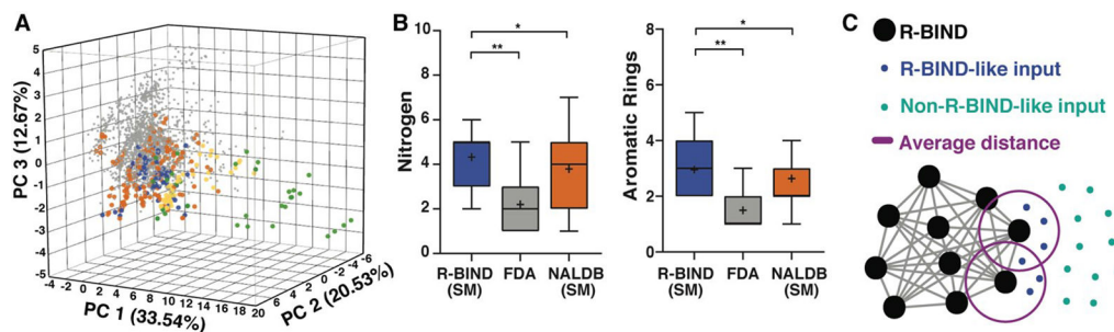
Figure 4. RNA-targeted Bioactive LigaNd Database (R-BIND) reveals distinct properties of RNA-targeted small molecules.
