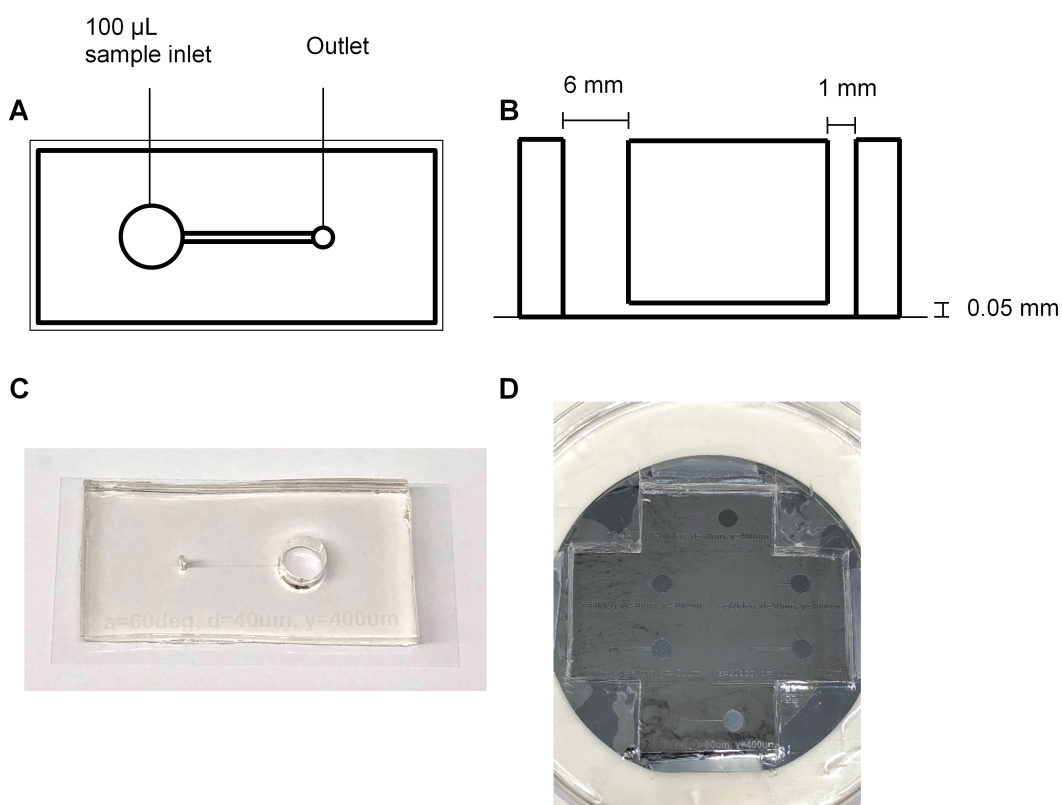
Figure 1. Fabrication of PDMS biochips. The PDMS biochip produced in this protocol features a 6 mm diameter inlet (well) which can hold up to 100 \mu l of sample, and a 1 mm diameter outlet which connects the channel to the pump. The channel has a length of 12 mm, width of 0.4 mm and a height of 0.05 mm (A, B, and C). The manufactured silicon wafer mask contains indentations which form the shape of the channel (D).
