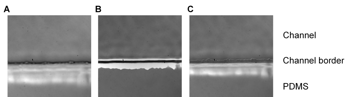
Figure 4. Planes of focus. Imaging of the biochip placed under an Olympus fluorescent microscope using a 60x objective. The plane of focus is displayed below the coverslip (A), above the coverslip (B) and on the coverslip (C). When the coverslip is in focus, the jagged edge of the PDMS (an artifact of the fabrication process) can be seen within the channel.
