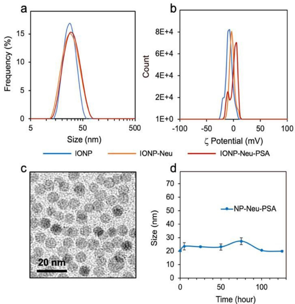
Fig. 4. Physicochemical properties of IONP-Neu-PSA. (a) Hydrodynamic sizes in 20 mM and (b) Zeta potentials of IONP, IONP-Neu, IONP-Neu-PSA. (c) TEM image of IONP-Neu-PSA. (d) Serum stability of IONP-Neu-PSA, characterized by incubating IONP-Neu-PSA in 10% FBS (v/v) supplemented cell culture medium at 37°C for 125 hrs and measuring hydrodynamic size of IONP-Neu-PSA over time. There is no significant change in size data over time as characterized by the two-tailed student's test ( p > 0.05 ).
