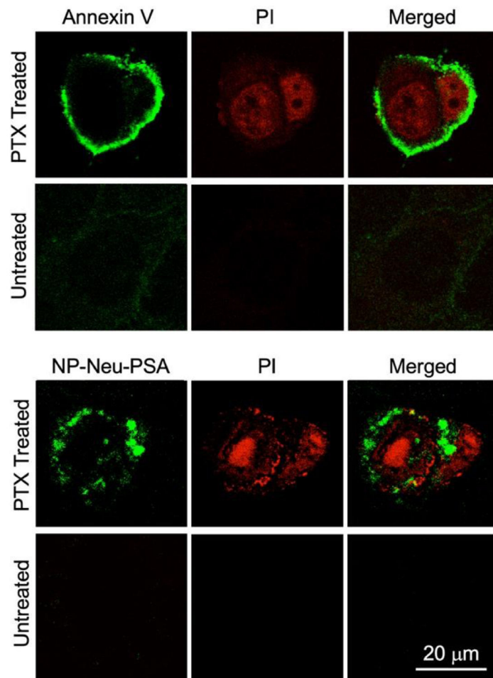
Fig. 7. In vitro apoptotic cell labeling characterized by confocal microscopy. 4T1 cells were either treated with 20 μM PTX for 24 hours to induced apoptosis or received no PTX treatment as control. Both the treated and untreated cells were labeled with PI (red), and either Annexin V-AF488 (green) or IO NP-Neu-PSA-Cy5 (green). All the stained 4T1 cells were then mounted onto glass slides with anti-fade agent.
