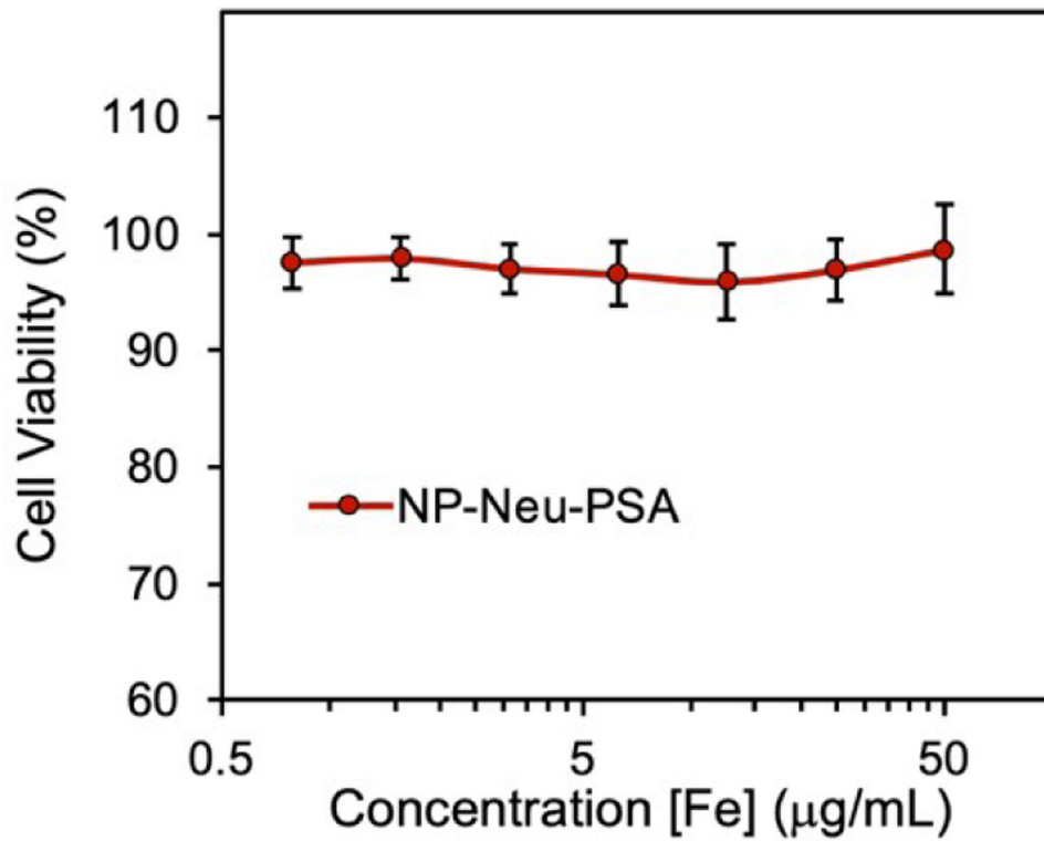
Fig. 5. Viability of 4T1 breast cancer cells treated with IONP-Neu-PSA at various concentrations. 4T1 cells were incubated with IONP-Neu-PSA for 72 hours at 37°C and 5% CO 2 . All the data points at various [Fe] concentrations show no significant difference from each other as characterized by the two-tailed student t test ( p > 0.05 ).
