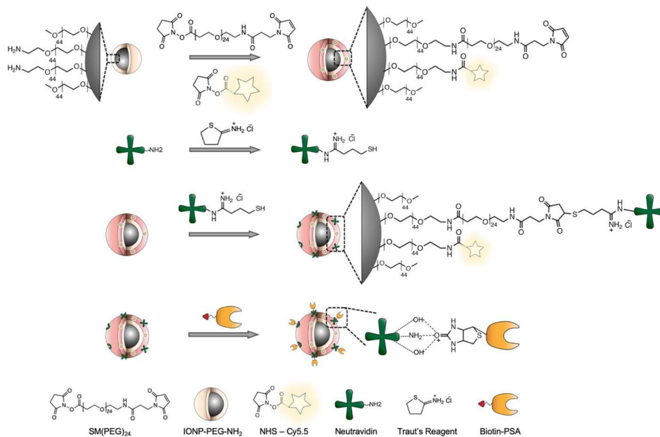
Fig. 1. Illustration of IONP-Neu-PSA synthesis. IONP-PEG-NH 2 was first functionalized with SM(PEG) 24 and NHS activated fluorophores. Thiolated neutravidin was conjugated onto IONP via SM(PEG) 24 bifunctional linker. Biotinylated PSA was then attached to neutravidin via avidin-biotin interaction.
