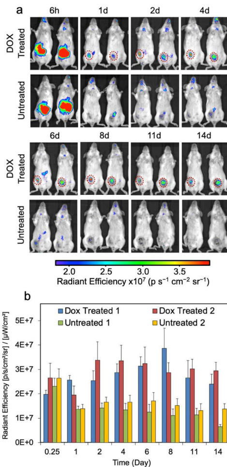
Fig. 8. In vivo monitoring of apoptosis. (a) Representative Near-IR images of two groups of tumor-bearing mice, with one group treated with DOX and another group receiving no treatment. Mice were monitored with IVIS for 14 days starting 6 hours post IONP-Neu-PSA-Cy5.5 injection. IONP-Neu-PSACy5.5 labeled apoptotic tumor regions are highlighted with a red dashed circle. The left and right mouse of the untreated group in each image are designated as Untreated 1 and Untreated 2, respectively. (b) Quantitation of the near-IR fluorescent intensity in (a). The left mouse and the right mouse in the Dox treated panel are assigned as Dox Treated 1 and Dox Treated 2 respectively.
