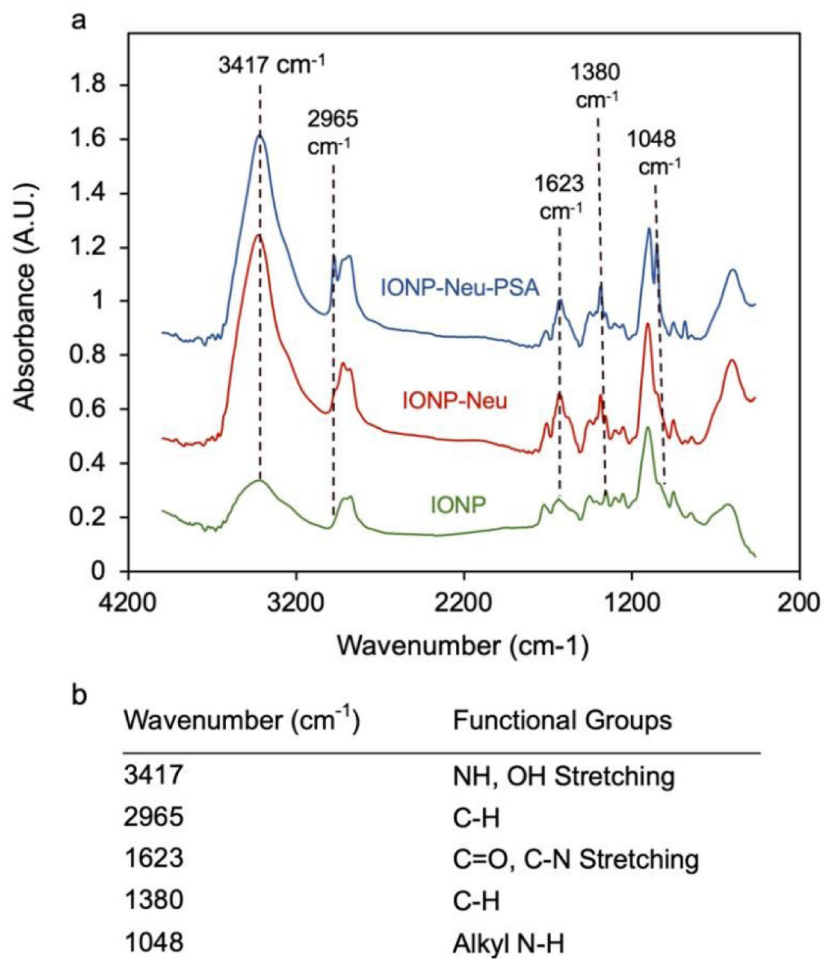
Fig. 2. NP bound PSA characterization and quantification. (a) FTIR absorbance spectrum analysis of IONP-Neu-PSA and IONP-Neu with IONP as the control particle. Peak wavenumbers unique to IONP-Neu and IONP-Neu-PSA are delineated with dashed lines. (b) Summary table of the wavenumbers of interest with their corresponding functional groups.
