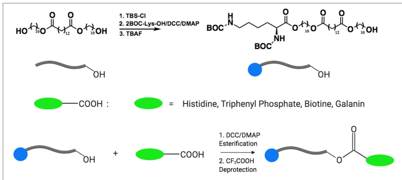
FIGURE 11 | Huang et al. (2018) prepared a series of asymmetric BAs. One of the polar head groups was fixed as lysine while the second was chosen from an assortment of functional polar moieties. Copyright 2018, Multidisciplinary Digital Publishing Institute.
