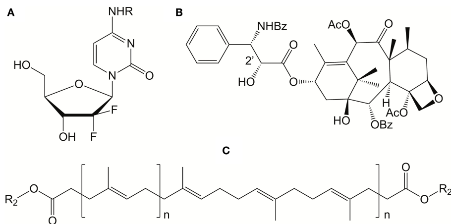
FIGURE 18 | Structures of anticancer drugs, gemcitabine ( A ) and paclitaxel ( B ), where R binds to the proposed hydrophobic squalene backbone ( C ). These “bolaform” prodrugs were shown to form nanoassemblies with in vitro activity on human and murine cancer cell lines. Reproduced from Caron et al. (2014), Royal Society of Chemistry.
