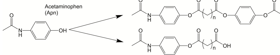
FIGURE 17 | Acetaminophen was modified into a bola-like structure. These amphiphilic derivatives self-assemble into hydrogels that can act as drug delivery platforms. Reproduced from Vemula et al. (2009), Elsevier.
