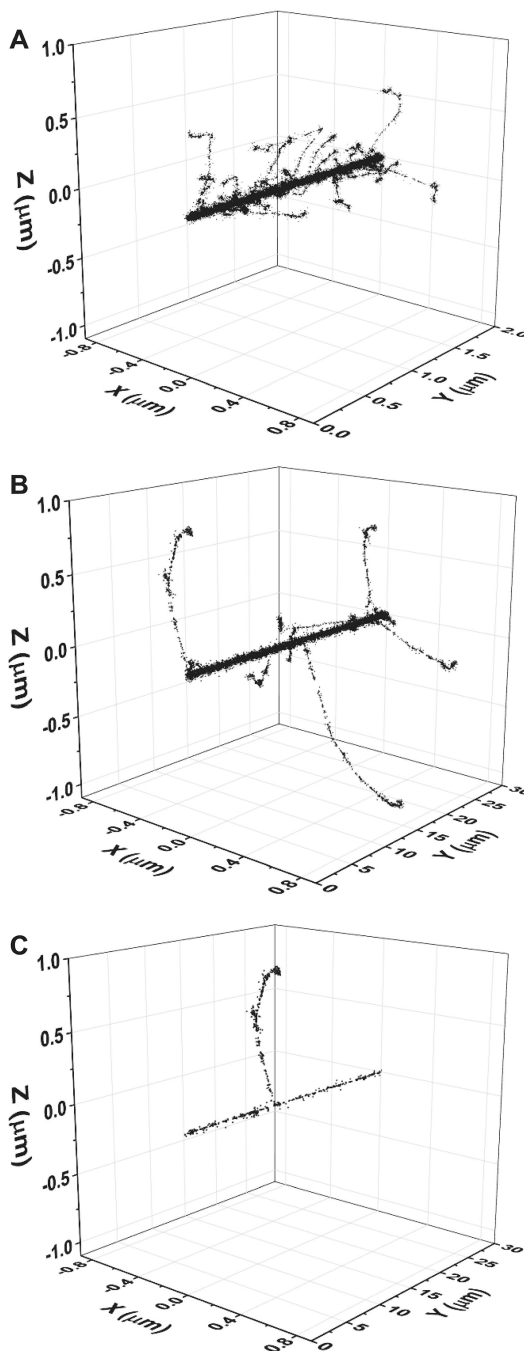
FIG. 2. Three-dimensional representations of track segments for the following impacting ions: (panel A) 4.1-MeV/nucleon ^{12}\text{C}^{6+} (LET \sim 330 keV/ \mu\text{m} , 2- \mu\text{m} track length), (panel B) 300-MeV/nucleon ^{12}\text{C}^{6+} (LET \sim 11 keV/ \mu\text{m} , 30- \mu\text{m} track length), and (panel C) 300-MeV ^1\text{H}^+ (LET \sim 0.3 keV/ \mu\text{m} , 30- \mu\text{m} track length) traversing through liquid water at 25°C, calculated (at \sim 10^{-13} s) with our IONLYS Monte Carlo simulation code. Ions are generated at the origin and start traveling along the y-axis. Each dot represents an interaction where energy deposition occurred. Surrounding the “core” of the track is a much larger region (named the
