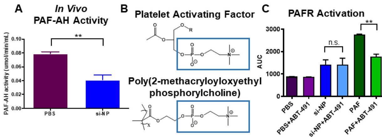
Figure 2. si-NPs stimulate PAF release, as measured through PAF-AH exhaustion, and do not directly agonize the PAF receptor.
