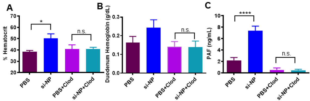
Figure 3. Pre-treatment with clodronate liposomes abrogates si-NP-related PAF elevation and toxicities.
