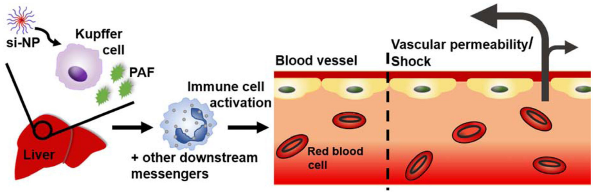
Figure 6. Schematic of proposed mechanism for PAF-mediated effects upon intravenous administration of nucleic acid nanocarriers.
