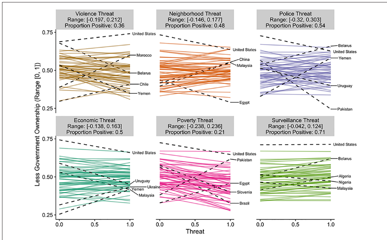
Figure 3. Estimated slopes between threat and less government ownership for each country.
