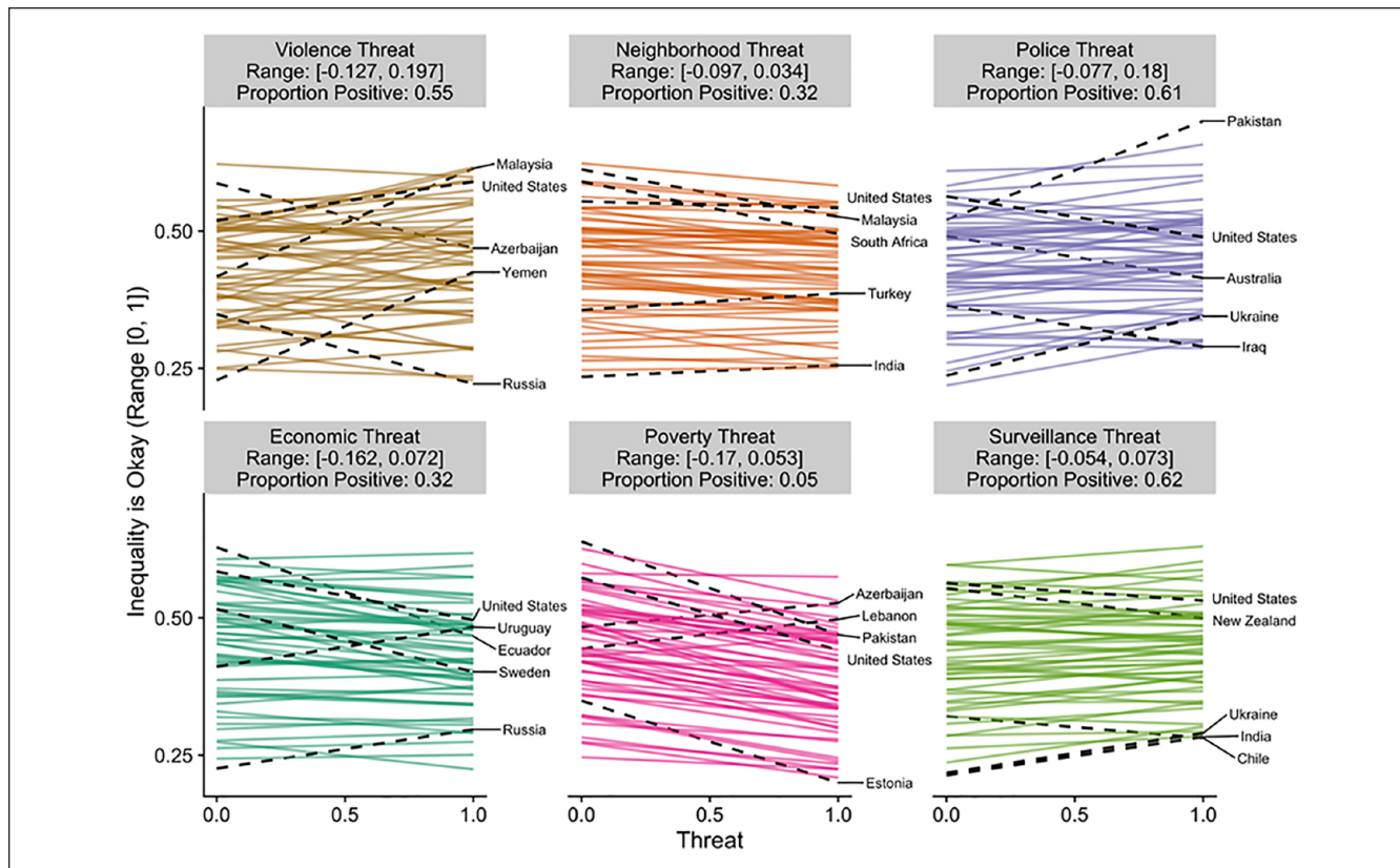
Figure 2. Estimated slopes between threat and inequality is okay for each country. Note. The two largest and two smallest slopes are highlighted and labeled. The United States is also highlighted and labeled for comparison purposes. See also Table S5.
