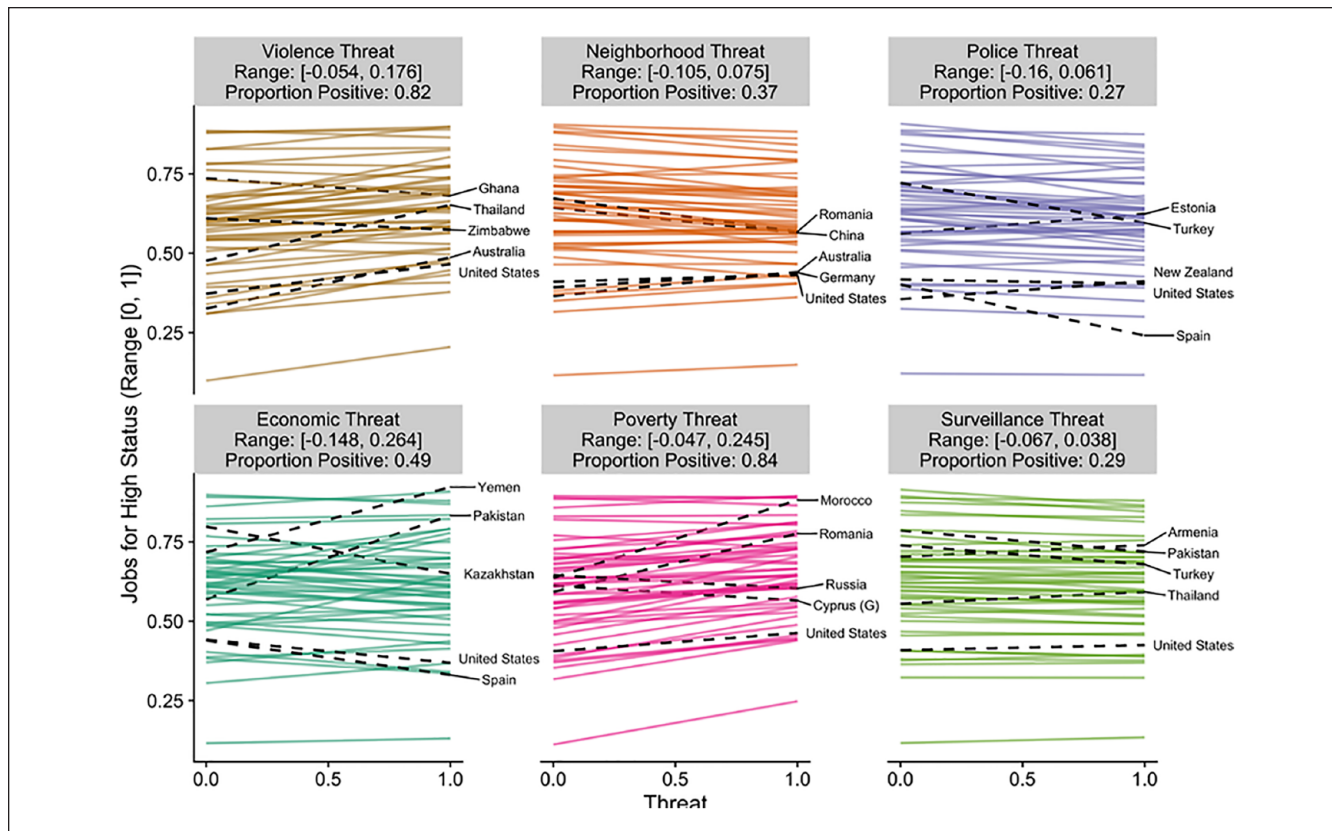
Figure 4. Estimated slopes between threat and jobs for high status for each country. Note. The two largest and two smallest slopes are highlighted and labeled. The United States is also highlighted and labeled for comparison purposes. See also Table S7.
