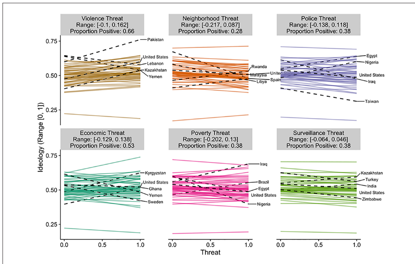
Figure 6. Estimated slopes between threat and ideological identification for each country. Note. The two largest and two smallest slopes are highlighted and labeled. The United States is also highlighted and labeled for comparison purposes. See also Table S9.
