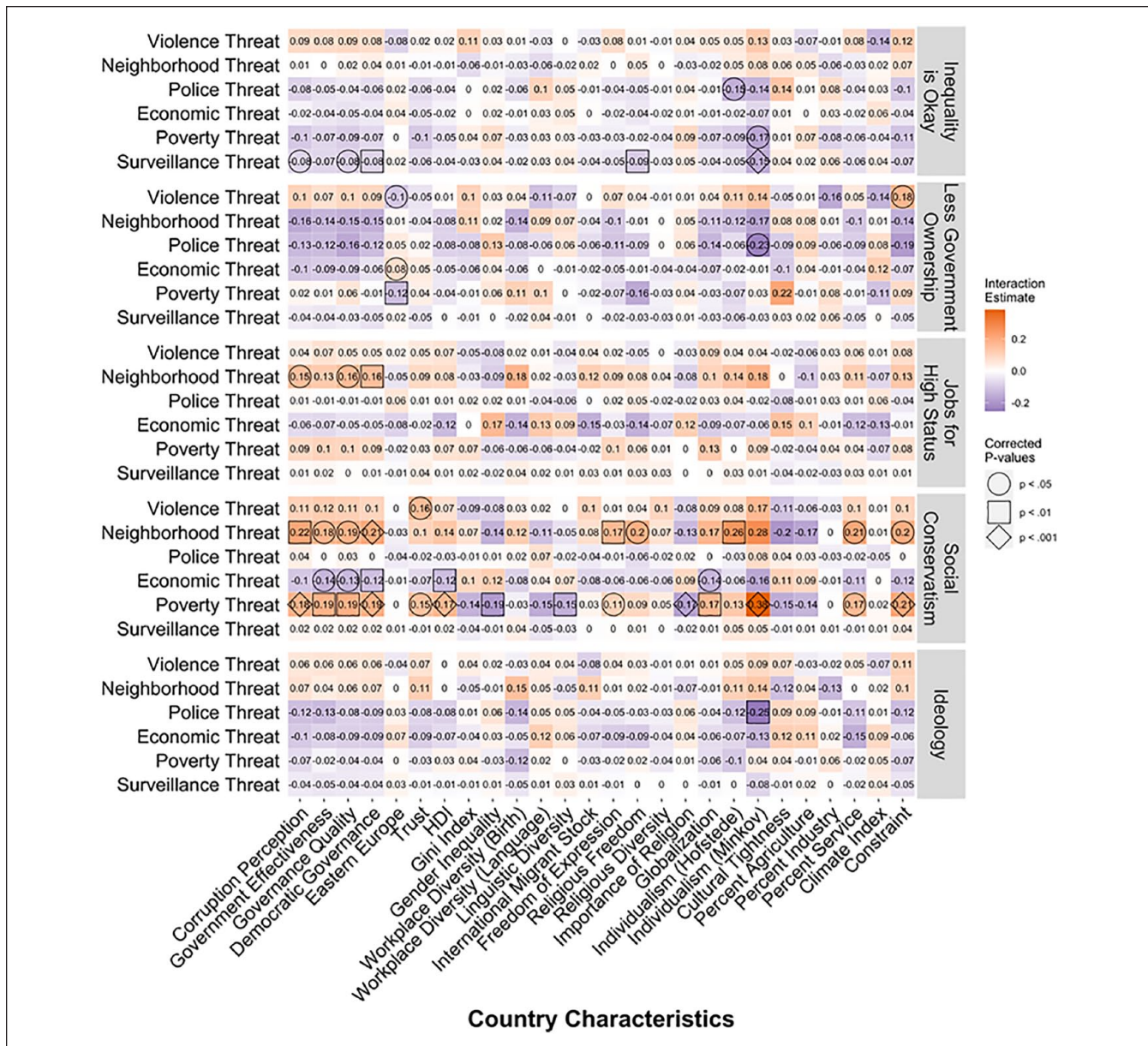
Figure 7. Estimates for the interaction between-ountry characteristics (x-axis) and threats (y-axis) for the five measures of political beliefs (row chunks).
