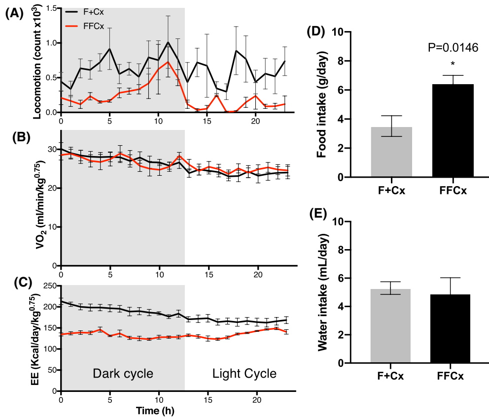
FIGURE 5 Metabolic energy profile and dietary intake for male mice at 24 weeks. Experimental (FFCx) mice were placed in a metabolic cage and compared with control littermates in another cage for each trial over one d with the indicated dark/light cycle. A, Locomotion activity (arbitrary units). B, Normalized oxygen consumption rate. C, Energy expenditure. Food intake (D) and water intake (E) were also measured over 24 hours. Statistical analysis was by Student's t test, with only P-values expressing significance below 0.05 being reported. Bars represent mean \pm SE. Numbers of animals used for each genotype: FFCx 14 and F + Cx 14
