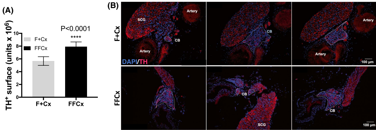
FIGURE 1 Quantitative assessment of TH expression in the CB of mice at 72 weeks. A, TH + area (arbitrary units) in carotid bifurcations based on analysis of nine TH-Cre experimental (FFCx) and nine control (F + Cx) mice. Statistical analysis used a Student's t test where significance is reported for P -values below .05. Bars represent mean ± SEM. B, Example immunofluorescent staining shows TH (red) and DAPI (blue) where the discontinuous white line outlines the CB regions in each section
