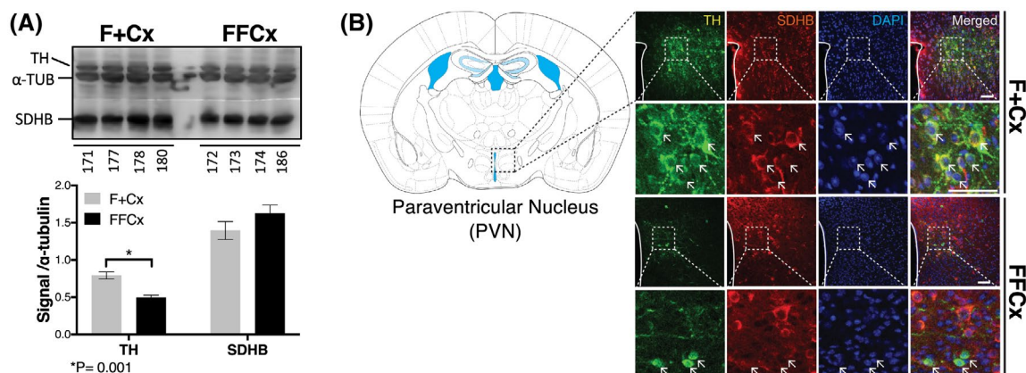
FIGURE 6 Changes in TH + cells in key regions of the hypothalamus important for feeding behavior. A, Western blot analysis of TH and SDH (represented by SDHB) in hypothalamic preoptic tissue for the indicated four representative animals. Western blot signal quantitation statistics were analyzed using a Student's t test with bars indicating mean \pm SD. B, Fluorescent immunohistochemical staining analysis of the PVN monitoring TH (green), SDHB (red), and DAPI (blue) Arrows indicate example cells showing contrasting features. Scale bar: 50 \mu m
