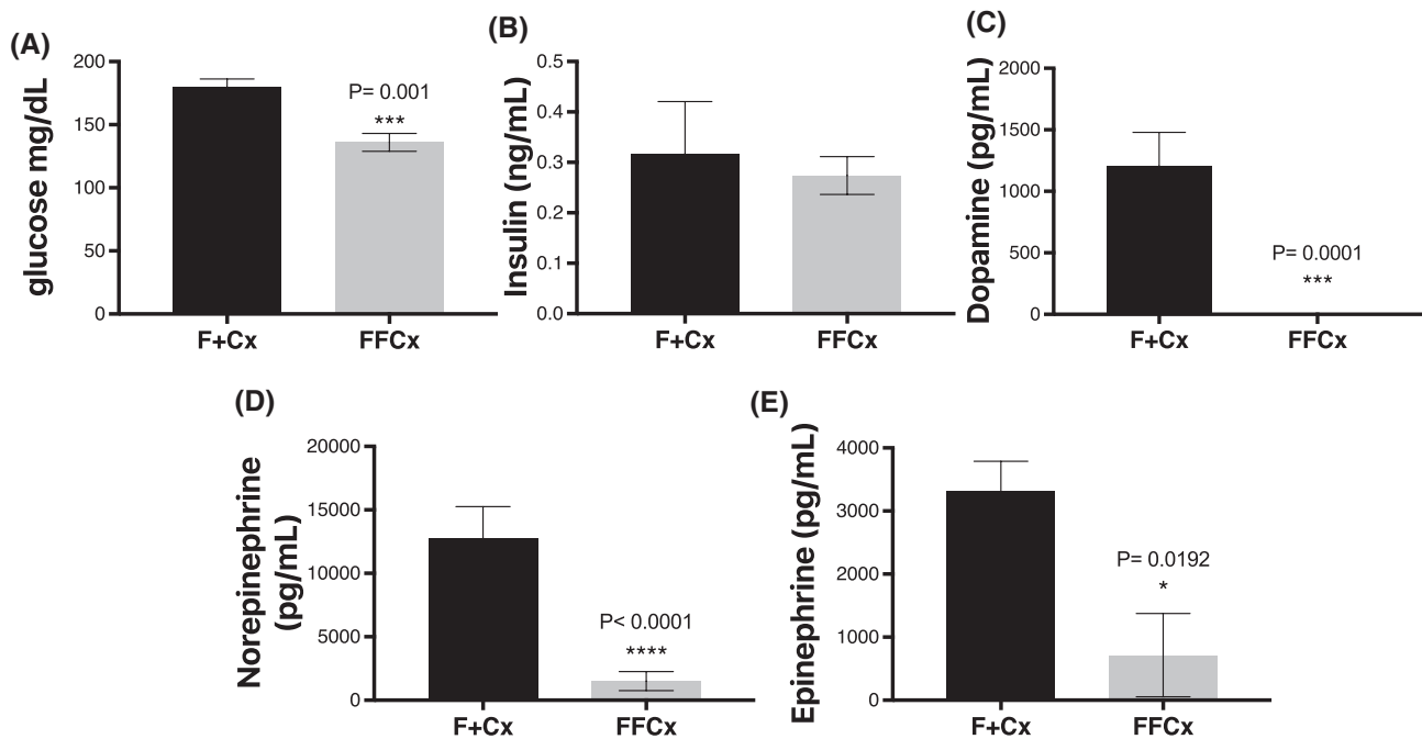
FIGURE 7 Blood glucose, insulin, and catecholamines for male mice at 24 weeks. Mice were fasted for 4 hours prior to serum collection. A, Tail vein whole blood was used to monitor glucose using an Alpha TRAK 2 monitoring kit. B-E, Serum was analyzed to measure insulin and the indicated hormones. Statistical analysis was by Student's t tests, with only P values below .05 indicated and measurements below the detection limit were substituted with the lowest detectable level of each assay divided by 2^{1/2} , as described (Ogden, 2010). Bars indicate mean \pm SE. Data represent seven male mice per group
