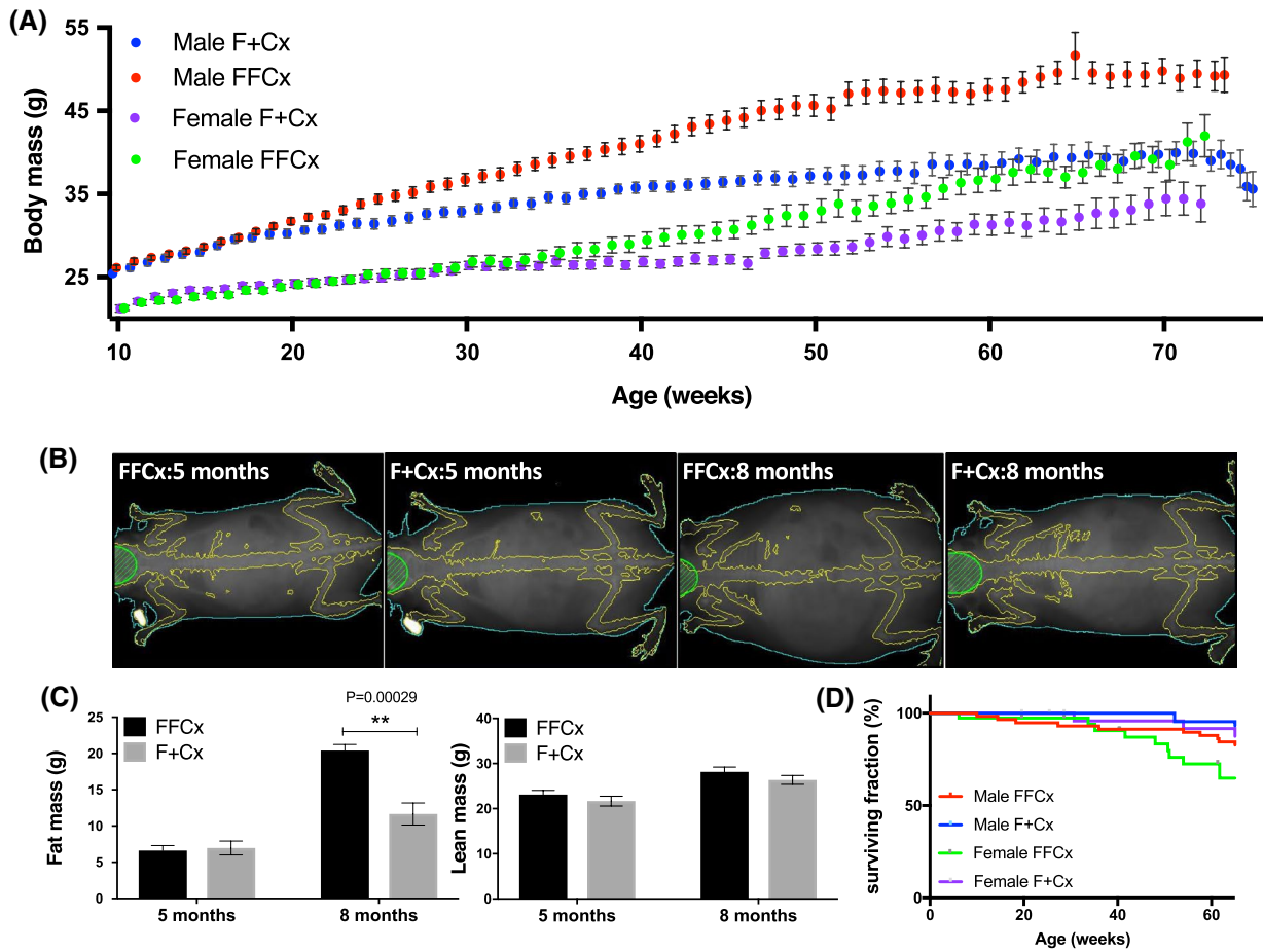
FIGURE 3 Obesity in experimental mice upon SDHC loss in TH + cells. A, Body weight over 78 weeks. Numbers of mice for each genotype were: 36 FFCx and 30 F + Cx males; 28 FFCx and 30 F + Cx females. B, X-ray imaging of representative mice at 20 (preobese) and 32 (obese) wk using densitometry with dual energy X-ray absorptiometry (DEXA) in a Lunar PIXImus scanner. C, Fat and lean mass for seven experimental and seven control mice at 20 and 32 weeks. D, Survival of mice represented in panel A. Statistical analyses were performed using Prism 8 with bars indicating mean \pm SD. Fat and lean mass data were analyzed by two-way ANOVA with Tukey's correction test over genotype and time
