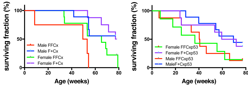
FIGURE 2 Survival of mice of the indicated genotypes maintained under chronic hypoxia (10% O 2 ). A, Lifespan data for mice of the indicated SDHC TH-Cre genotypes over 80 weeks. Data represent 23 FFCx and 18 F + Cx males; 16 FFCx and 16 F + Cx females. B, Lifespan data for mice of the indicated genotypes expressing a dominant negative p53 allele in TH + cells over 80 weeks. Data represent 14 FFCx and 14 F + Cx males; 15 FFCx and 14 females. Data analysis was conducted in Prism 8
