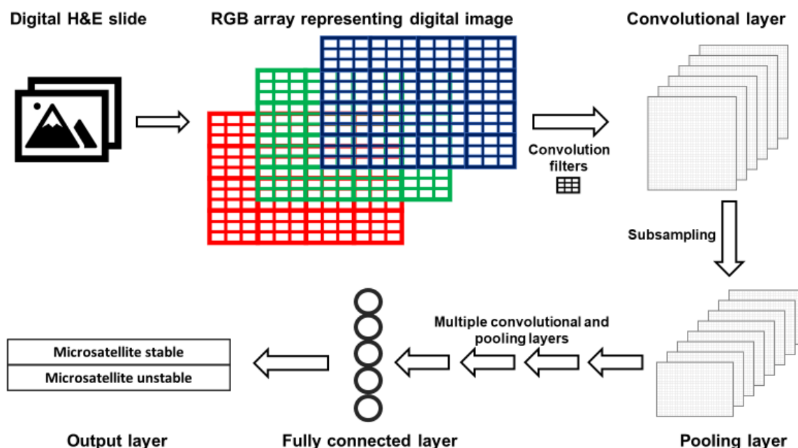
Figure 2. Simplified architecture of a convolutional neural network (CNN). Images acquired with digital pathology are composed of pixels. The color of each pixel can be represented with values of the red, green and blue (RGB) scheme. RGB arrays are subjected to filters to create a convolutional layer. Filters detect specific features from an image (e.g., lines, edges). A pooling layer with a reduced number of parameters is created by summarizing (subsampling) the input of the convolutional layer. After a defined number of convolutional and pooling layers, fully connected layers are created. Fully connected layers are uni-dimensional layers from which the output is predicted.
