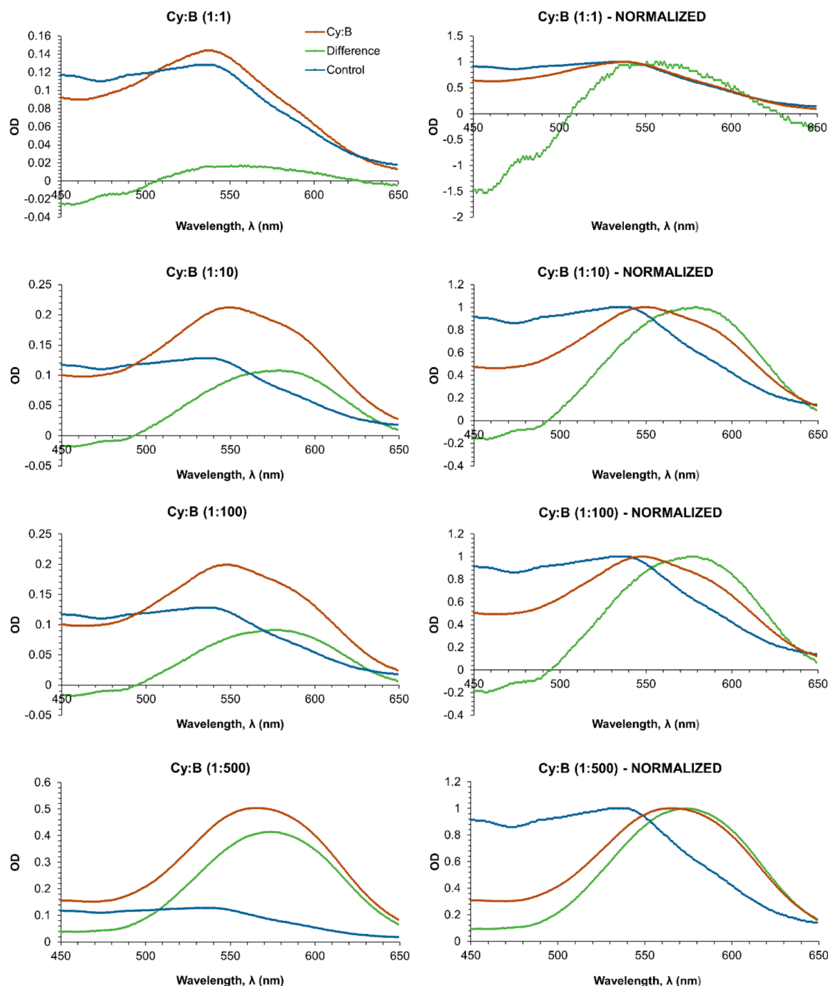
Figure 5. UV–vis spectra of cyanidin-based anthocyanins solutions containing B at the various Cy:B ratios explored (red curves), at pH 5. The curves (green) resulting from subtracting the control solution (blue curves) spectrum (left) are also shown. Normalized curves (right) are also shown to more clearly note bathochromic shifts.
