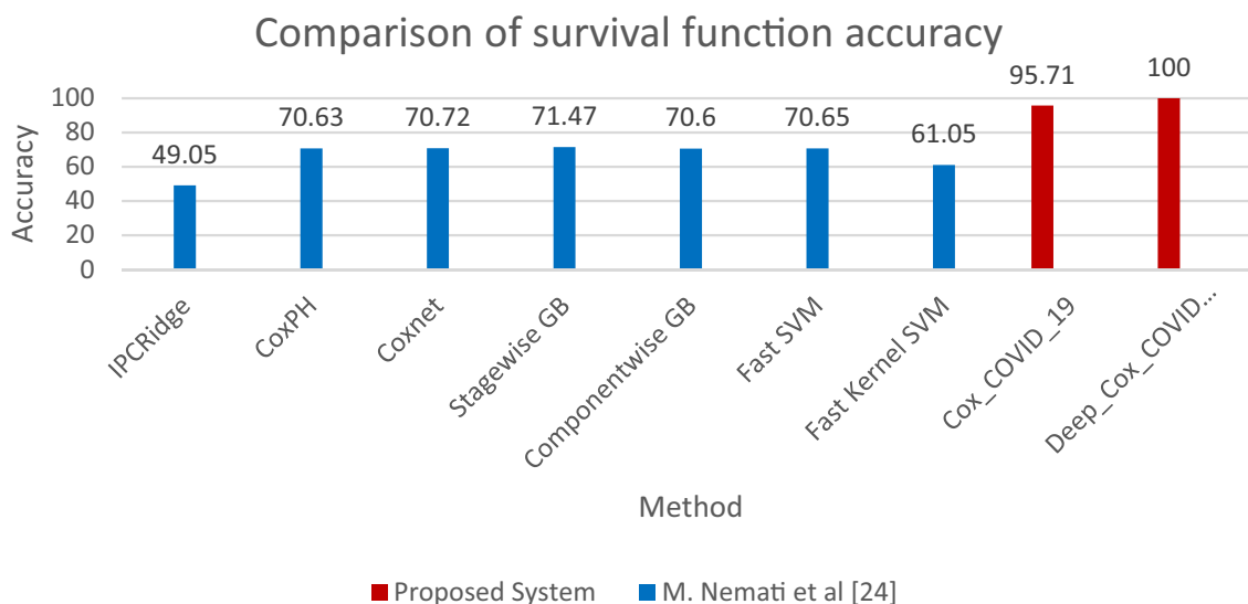
Fig. 7 Survival function accuracy for proposed system and other algorithms
