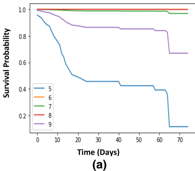
Fig. 5 a, and b: Survival curve for randomly 10 patients using Cox_COVID_19
