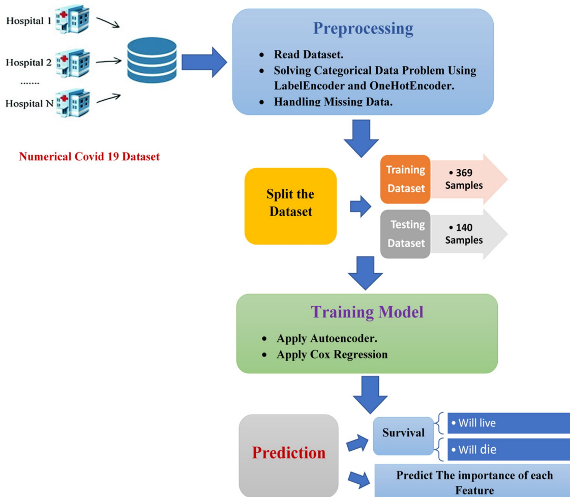
Fig. 3 Proposed survival analysis system architecture
