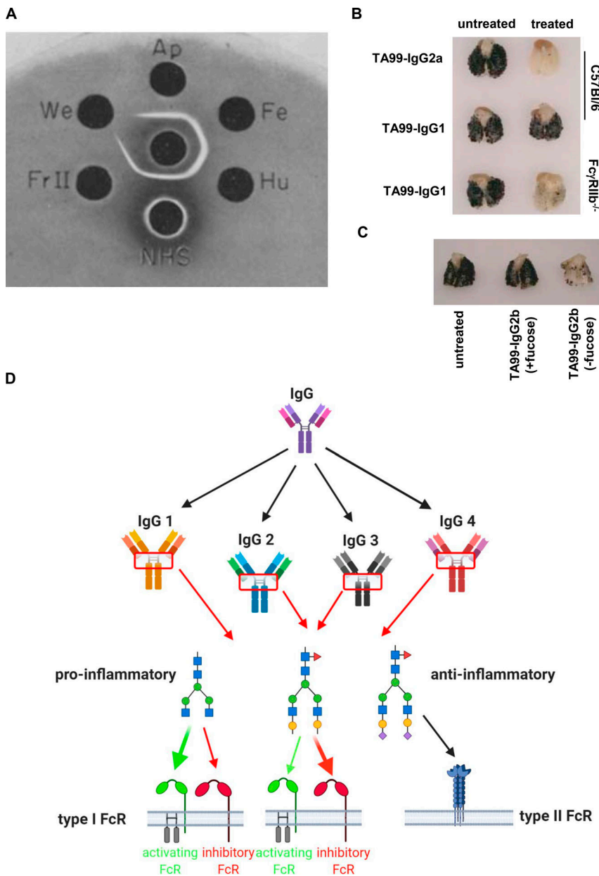
The complexity of IgG subclass activity. (A) Shown is an in-gel antibody precipitation assay (ouchterlony assay) from Grey and Kunkel (1964), demonstrating that a rabbit antiserum generated against one myeloma IgG molecule precipitates some but not all IgG antibodies derived from other multiple myeloma patients (IgG from patient We is not precipitated, whereas IgG from patients Ap, Fe, Hu, and FrII is precipitated). The antiserum also reacted against normal human serum demonstrating the presence of IgG subclasses in healthy individuals. (B) Depicted are lung melanoma metastases in C57BL/6- and FcγRIIb-deficient mice left untreated or treated with IgG subclass switch variants (IgG1 and IgG2a) of the melanoma-specific antibody TA99. (C) Shown are lung melanoma metastases in C57L/6 mice left untreated or treated with a TA99-IgG2b subclass variant carrying a sugar moiety with or without fucose in its Fc domain. (D) Schematic representation of factors influencing IgG activity. Apart from individual IgG subclasses, IgG glycosylation plays a major role in balancing the pro- and anti-inflammatory activities of IgG via modulating the interaction with type I and type II Fc-receptors (FcR). See text for further details.
