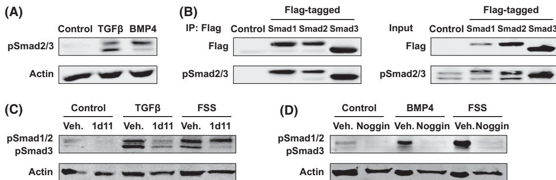
FIGURE 4 FSS-mediated activation of TGF \beta and BMP R-Smads require their corresponding ligand. A, Representative western analysis of control or ligand-treated cells grown in culture dishes revealing independent regulation of pSmad bands. B, Anti-Flag co-immunoprecipitation (left panels) or western (Input, right panels) of lysates from control or Flag-Smad transfected OCY454 cells, followed by corresponding western analysis with antibodies against Flag or pSmad2/3. C, D, Representative western analysis of cells pretreated (60 minutes) with vehicle, 1d11 TGF \beta -blocking antibody (C), or the BMP ligand antagonist Noggin (D) followed by stimulation (30 minutes) with TGF \beta (5 ng/mL), BMP4 (50 ng/mL), or FSS (0.1 Pa) with Smads labeled as identified in B
