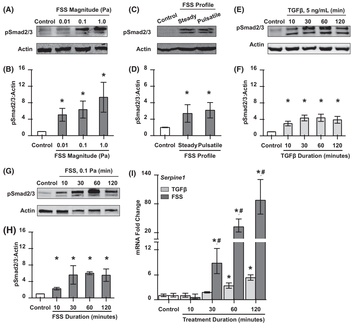
FIGURE 2 TGF \beta and FSS exhibit overlapping, but distinct, responses in OCY454 cells. A-H, Western analysis and quantification of Smad phosphorylation in OCY454 cells grown in control conditions or following stimulation with steady or pulsatile (1 s on, 1 s off) FSS for 30 minutes as labeled (A-D), or a time course of TGF \beta treatment (E, F) or FSS stimulation (G, H). FSS profile is steady unless otherwise indicated. I, qRT-PCR analysis of TGF \beta pathway target gene Serpine1 in control, TGF \beta -treated, or FSS-stimulated cells. All values normalized to control cells. * P < .05 compared to unstimulated cells and # P < .05 compared to TGF \beta -treated cells
