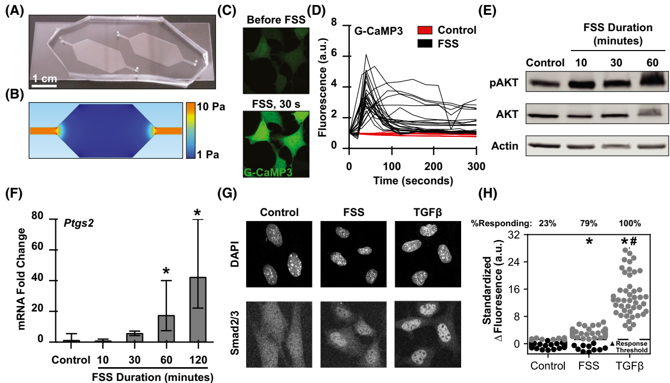
FIGURE 1 FSS rapidly induces nuclear translocation of Smad2/3 in OCY454 cells. A, B, Fluid flow through the elongated hexagonal polydimethylsiloxane (PDMS) microfluidic chambers designed and used in FSS experiments was modeled using COMSOL. C, D, Images and fluorescence intensity quantification of individual OCY454 cells transfected with the calcium reporter G-CaMP3 prior to and following stimulation with 0.1 Pa FSS, normalized to initial cellular intensity ( n = 3-6 biological replicates). E, Western analysis of AKT phosphorylation following stimulation with 0.1 Pa FSS. F, qRT-PCR analysis of mechanoresponsive gene Ptgs2 following stimulation with 1 Pa FSS, normalized to control cells. G, Representative images of Smad2/3 nuclear localization in control cells or following 30-minute treatments with FSS (0.1 Pa) or TGF \beta (5 ng/mL). H, Fluorescence quantification on individual OCY454 cells showing differences in (nuclear-cytosolic) Smad2/3 intensity and %responding cells per condition (standardized to controls, n = 3 biological replicates). * P < .05 compared to unstimulated cells and # P < .05 compared to FSS-stimulated cells
