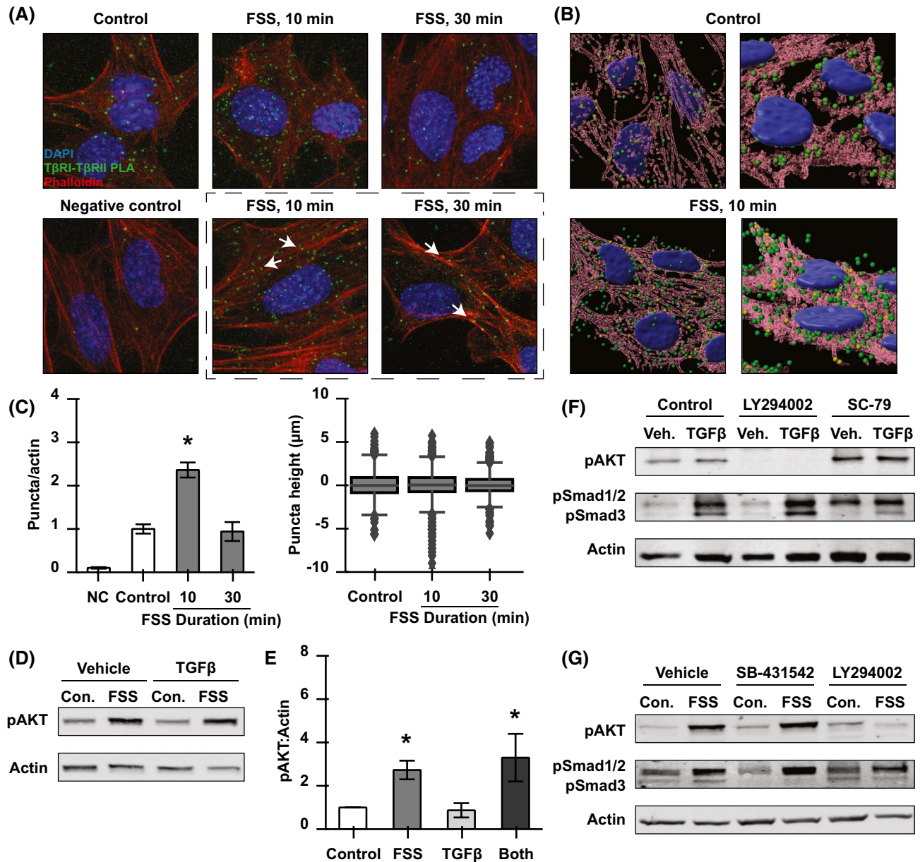
FIGURE 7 FSS-dependent regulation of TGF \beta receptor heteromerization. A, Images of proximity ligation assay (PLA) between T \beta RI and T \beta RII ( n = 5 regions of interest). Dashed lines show puncta localization relative to Actin fibers. B, C, IMARIS analysis of images (B) allows quantitative analysis of puncta frequency and spatial distribution in the presence or absence of FSS (C). D, E, Western analysis and quantification of control cells and cells treated with TGF \beta or stimulated with FSS (30 minutes). F, Representative western analysis from cells pretreated (60 minutes) with vehicle or a PI3K/AKT inhibitor (LY294002) or agonist (SC-79) followed by treatment with TGF \beta (30 minutes). G, Representative western analysis from cells pretreated (60 minutes) with vehicle or a T \beta RI or PI3K/AKT inhibitor followed by treatment (30 minutes) with 0.1 Pa FSS. All values normalized to control cells. * P < .05 compared to unstimulated cells
