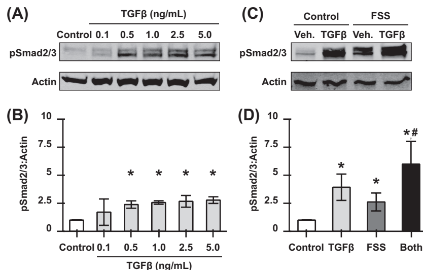
FIGURE 3 Concurrent stimulation with FSS and TGF \beta results in higher levels of phosphorylated Smads than either treatment alone. A, B, Western analysis and quantification of control or TGF \beta -treated OCY454 cells grown in cell culture dishes for 30 minutes, normalized to control cells. C, D, Western analysis and quantification of OCY454 cells grown in microfluidic devices in the absence of stimulation or following 30-minute treatment with TGF \beta (5 ng/mL) and/or FSS (0.1 Pa). All values normalized to control cells. * P < .05 compared to unstimulated cells and # P < .05 compared to FSS-stimulated group
