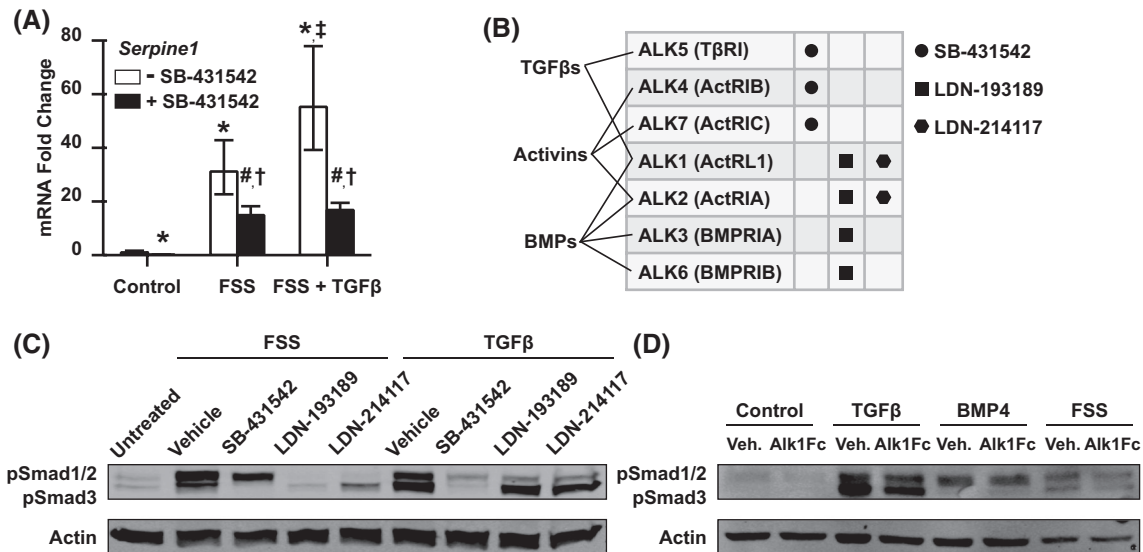
FIGURE 5 FSS stimulation activates multiple distinct TGFβ family type I receptors in OCY454 cells. A, qRT-PCR analysis of TGFβ target gene Serpine1 after 60-minute treatment with vehicle or SB-431542 followed by 120-minute treatment with TGFβ or FSS stimulation as indicated (n = 4 biological replicates). All values normalized to control cells. * P < .05 compared to unstimulated cells and # P < .05 compared to SB-treated controls; † P < .05 compared to corresponding treatment group without SB-431542, ‡ P < .05 compared to FSS-stimulated cells. B, C, Representative western analysis of Smad phosphorylation in control cells and cells pretreated (60 minutes) with vehicle or an inhibitor of a subset of TGFβ type I receptors (SB-431542, ALK4/5/7 inhibitor; LDN-193189, ALK1/2/3/6 inhibitor; LDN-214117, ALK1/2 inhibitor, as shown in B), followed by treatment (30 minutes) with TGFβ or FSS (C) (n = 3 biological replicates). D, Representative western analysis of cells pretreated (60 minutes) with ALK1Fc followed by treatment (30 minutes) with TGFβ, BMP4, or FSS (n = 2 biological replicates, non-flow conditions were collected from cells grown in well plates)
