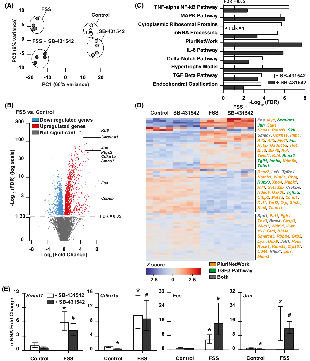
FIGURE 6 RNA-seq analysis supports potent FSS regulation of TGFβ superfamily signaling. A, Principal component analysis of sample variation considering the 500 genes with greatest variance. B, Volcano plot showing the distribution of differential gene expression in FSS-stimulated and unstimulated cells, and identifying induced (red) and repressed (blue) differentially expressed genes (DEGs). C, Enrichr pathway analysis using the WikiPathways database reveals the top ten most significantly regulated pathways, including TGFβ, that remain significantly regulated even in the presence of SB-431542. D, Genes related to the TGFβ and PluriNetWork pathways were clustered in a heatmap, and genes in each cluster are grouped. E, qRT-PCR analysis of established TGFβ-inducible genes Smad7 , Cdkn1a , Fos , and Jun following FSS stimulation in the presence or absence of SB-431542. Vehicle is 1% of DMSO. Dotted lines on graphs indicate threshold for statistical significance ( \text{FDR} < 0.05 ). * P < .05 compared to unstimulated cells and # P < .05 compared to SB-treated controls
