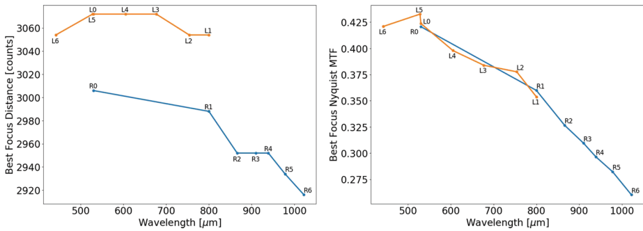
Fig. 29 Derived best focus position and MTF at Nyquist as a function of filter for a fixed target position. As in Fig. 25, a focus stack was taken for a fixed target position for each filter and the best-focus image was determined from the maximum measured MTF at Nyquist. Left: Comparison of the derived best focus motor position vs filter. For the visible band filters, we find a roughly constant focus position vs wavelength, resulting from the narrower range of wavelengths, suggesting a single autofocus frame can be acquired for all filters. For the near-IR filters, we find a systematic trend towards fewer motor counts for increasing wavelength. Right: Comparison of the derived best MTF value at Nyquist vs filter. For both cameras, we find a comparable decrease in MTF at Nyquist for increasing wavelength following the expected trend for decreased resolution with increasing wavelength resulting from the fixed effective aperture of the Mastcam-Z cameras
