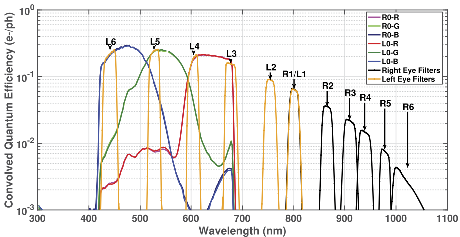
Fig. 44 Mastcam-Z Spectral Response ( r_{\lambda,k} ) for filters L0-L6 and R0-R6 in logarithmic space at a detector temperature of -5^\circ C . For the purposes of this plot, only the dominant RGB Bayer response is shown any given filter, except L0/R0
