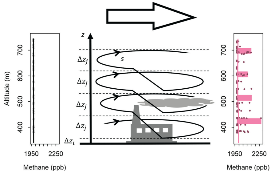
Figure 2. Illustration of the aircraft-based point source quantification approach, showing the flight direction ( s ) along with the heights of interpolated layers ( z_j ) and of the surface layer ( z_i ). Also shown are the vertical methane profiles for upwind and downwind sectors (dairy D; 28 January 2018). Points indicate individual methane observations, while the bars show the range in observed methane for each layer. Facility is not drawn to scale. For details, see text and the supporting information.
