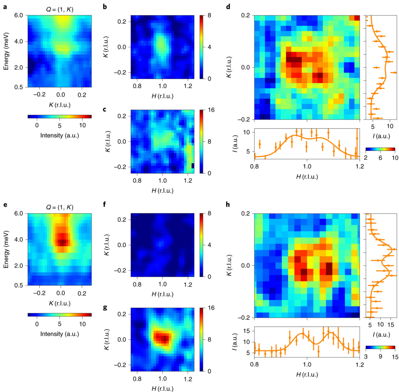
Fig. 2 |. Low-energy spin fluctuations in twinned FeSe below and above T_c .
