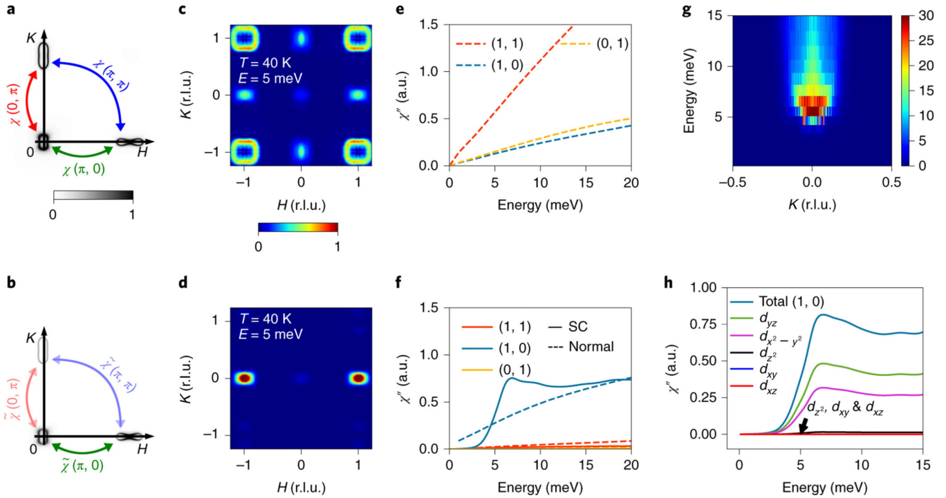
Fig. 5 |. Theoretical calculations of the spin fluctuations in detwinned FeSe.
