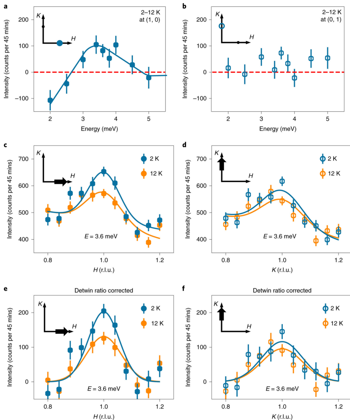
Fig. 4 | Effect of superconductivity on low-energy spin fluctuations of detwinned FeSe. a,b , Difference of the scattering in the superconducting state (below T_c ) and the normal state plotted as a function of energy for momentum transfers (1, 0) ( a ) and (0, 1) ( b ). The peak seen at E \approx 3.6 meV in a marks the neutron spin resonance. The solid blue and dashed red lines are guides to the eye. c , Wave-vector scans below and above T_c at E = 3.6 meV and (1, 0). d , Similar scans at (0, 1). e,f , (1, 0) ( e ) and (0, 1) ( f ) scans with background subtracted and detwinning ratio corrected (Supplementary Fig. 9). The solid lines in c-f are Gaussian
