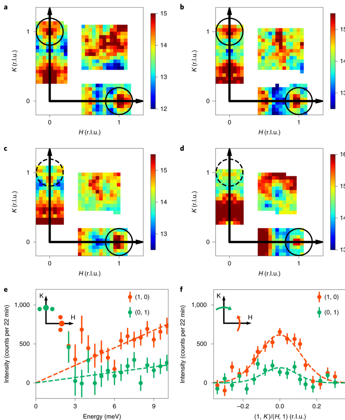
Fig. 3 | Normal-state spin fluctuations in detwinned FeSe.
