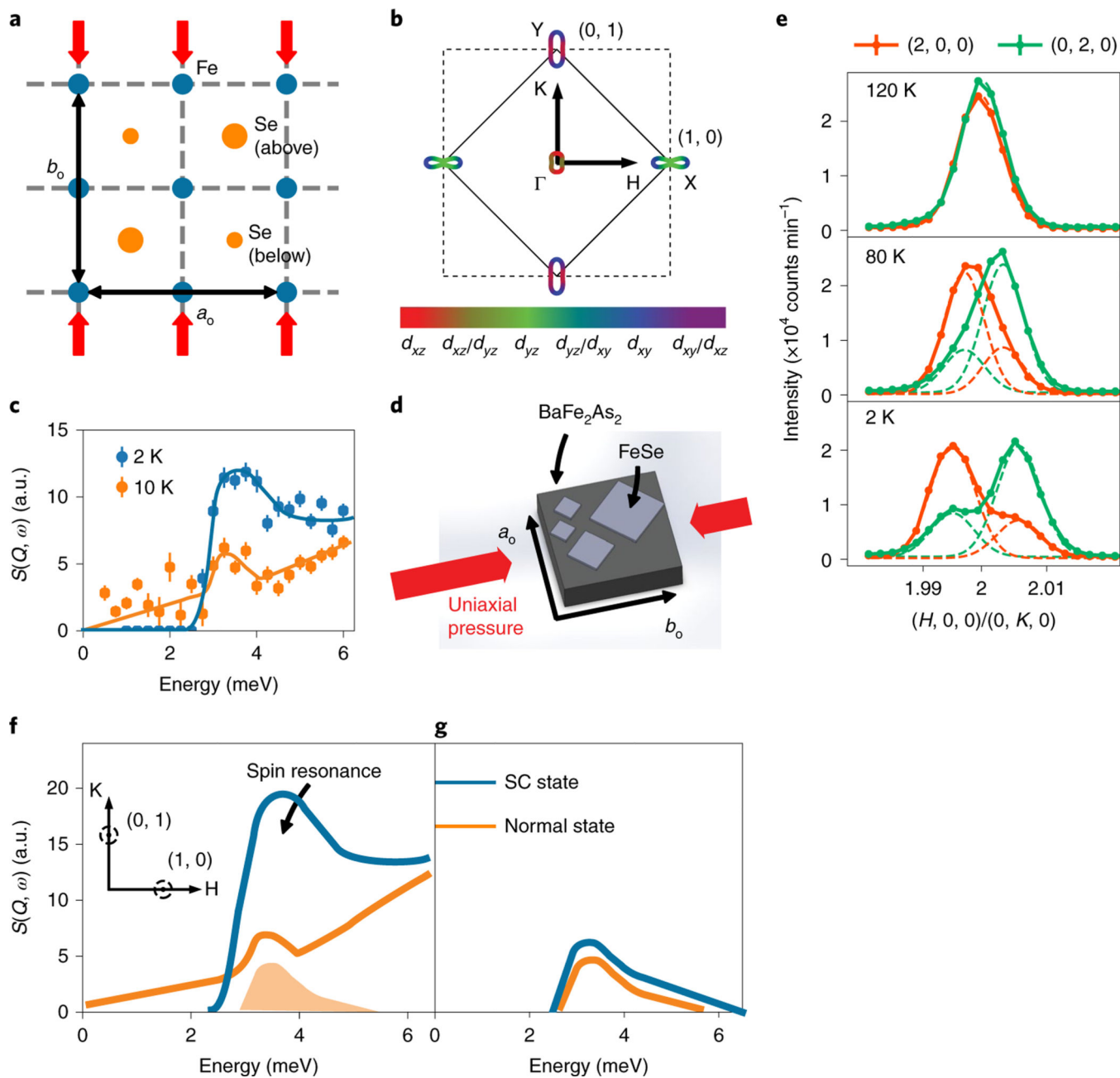
Fig. 1 | Crystal structure, Fermi surface and neutron scattering of FeSe.
