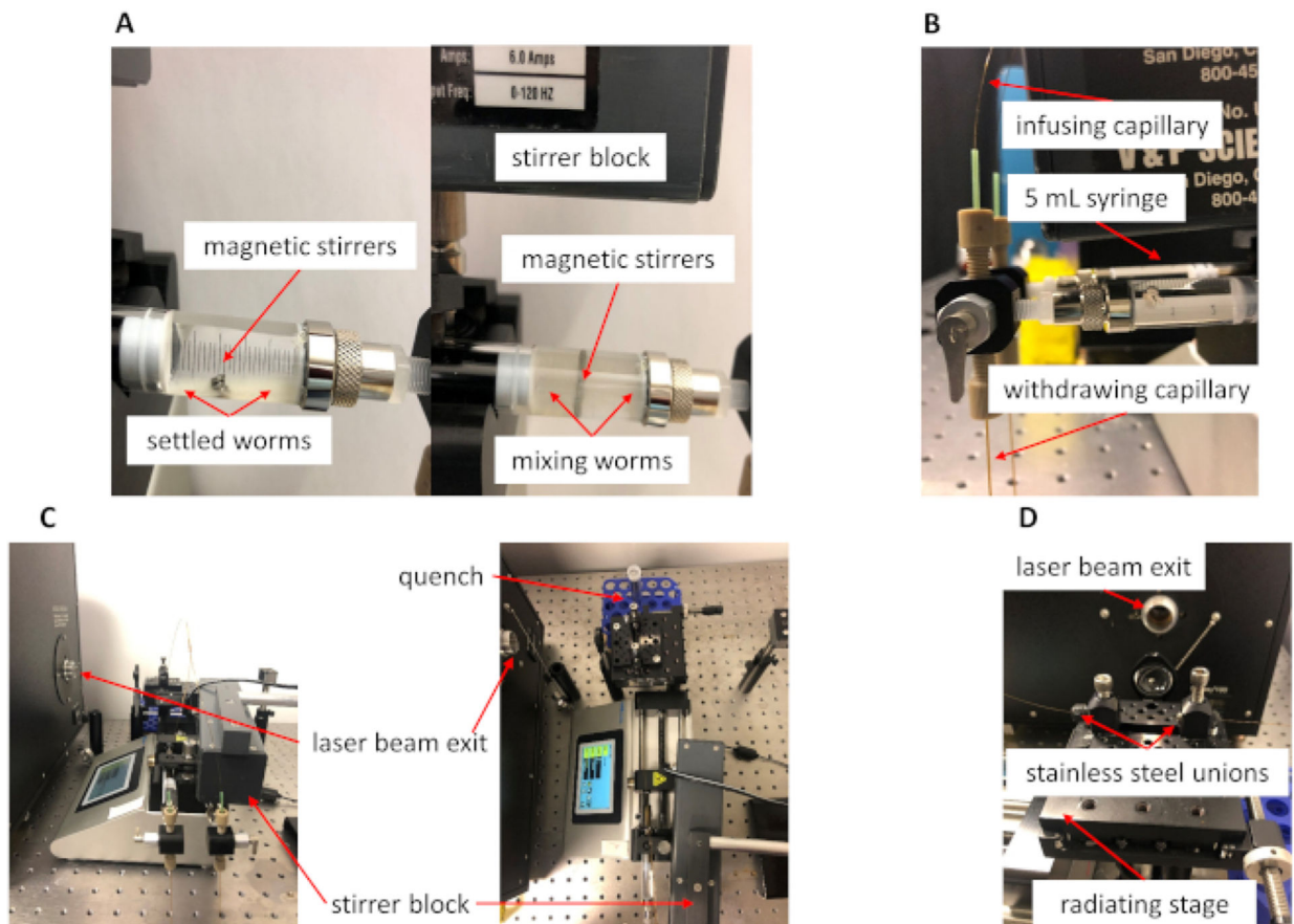
Figure 2. Microfluidic system during IV-FPOP.
