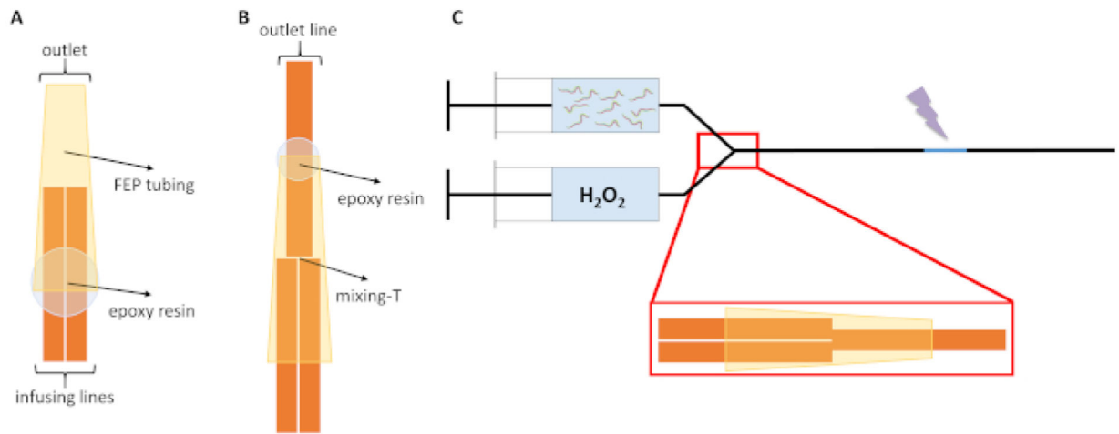
Figure 1. In vivo FPOP microfluidic flow system schematic.
