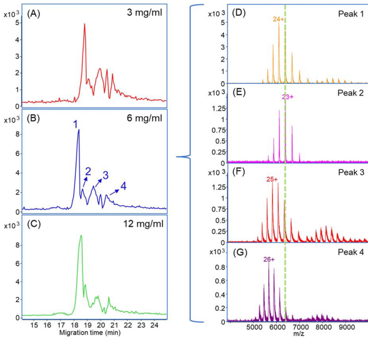
Figure 4. (A-C) Base peak electropherograms of native cIEF-assisted CZE-MS for 3, 6 and 12 mg/mL SigmaMAB; (D-G) Averaged mass spectra of the four major peaks separated in (B). Herein the LCP-coated capillary was used.
