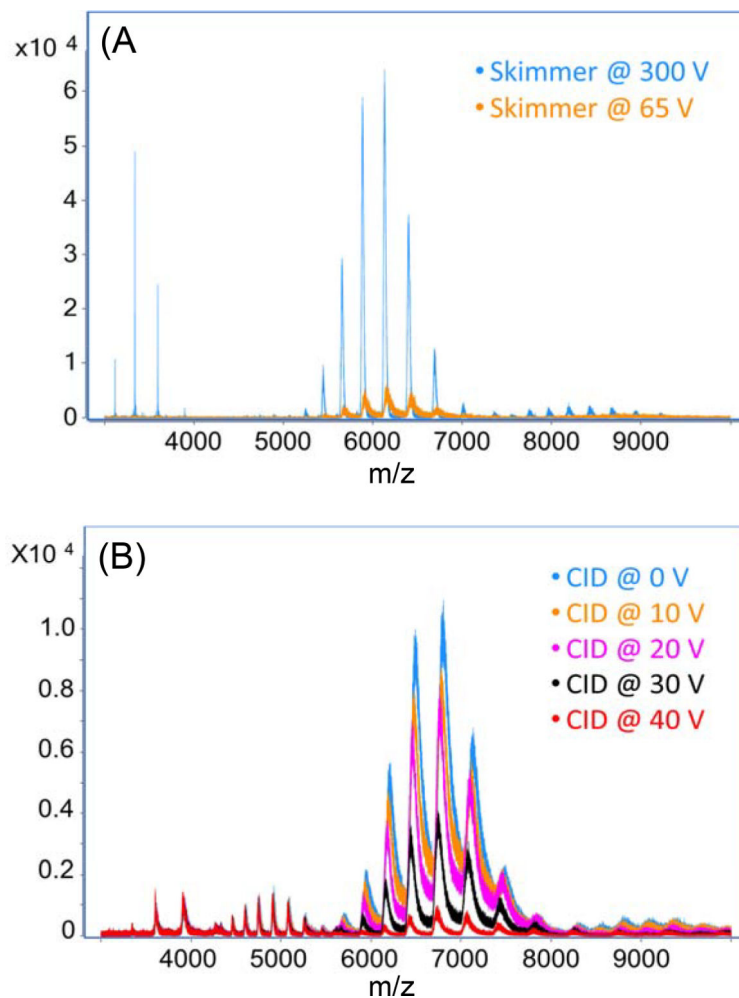
Figure 1. Mass spectra of the SigmaMAb through direct infusion MS with the CZE system and the nanospray sheathflow CE interface. (A) Skimmer and (B) Collision energy were investigated.
