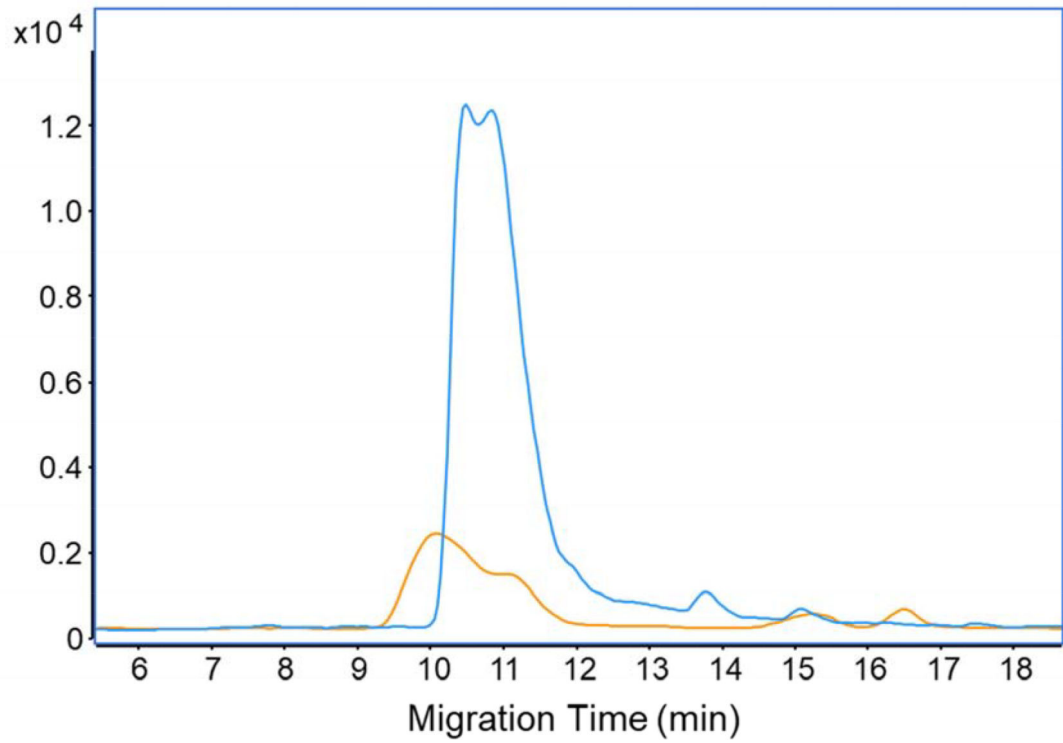
Figure 3. Base peak electropherograms of native CZE-MS for SigmaMAb with the LCP coated-capillary (blue) and the LPA coated-capillary (orange). Same MS settings and CZE conditions were applied for both CZE runs.
