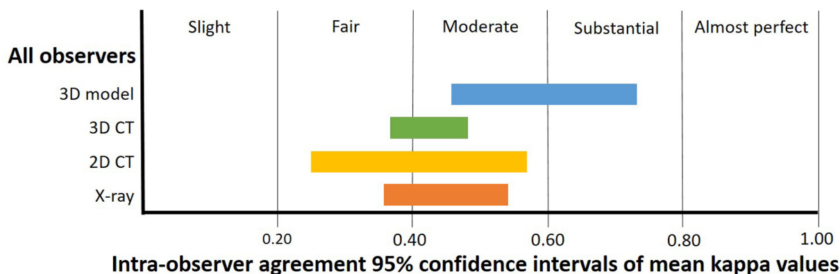
Figure 3 Intraobserver agreement using Landis and Koch criteria for each modality for all observers.
